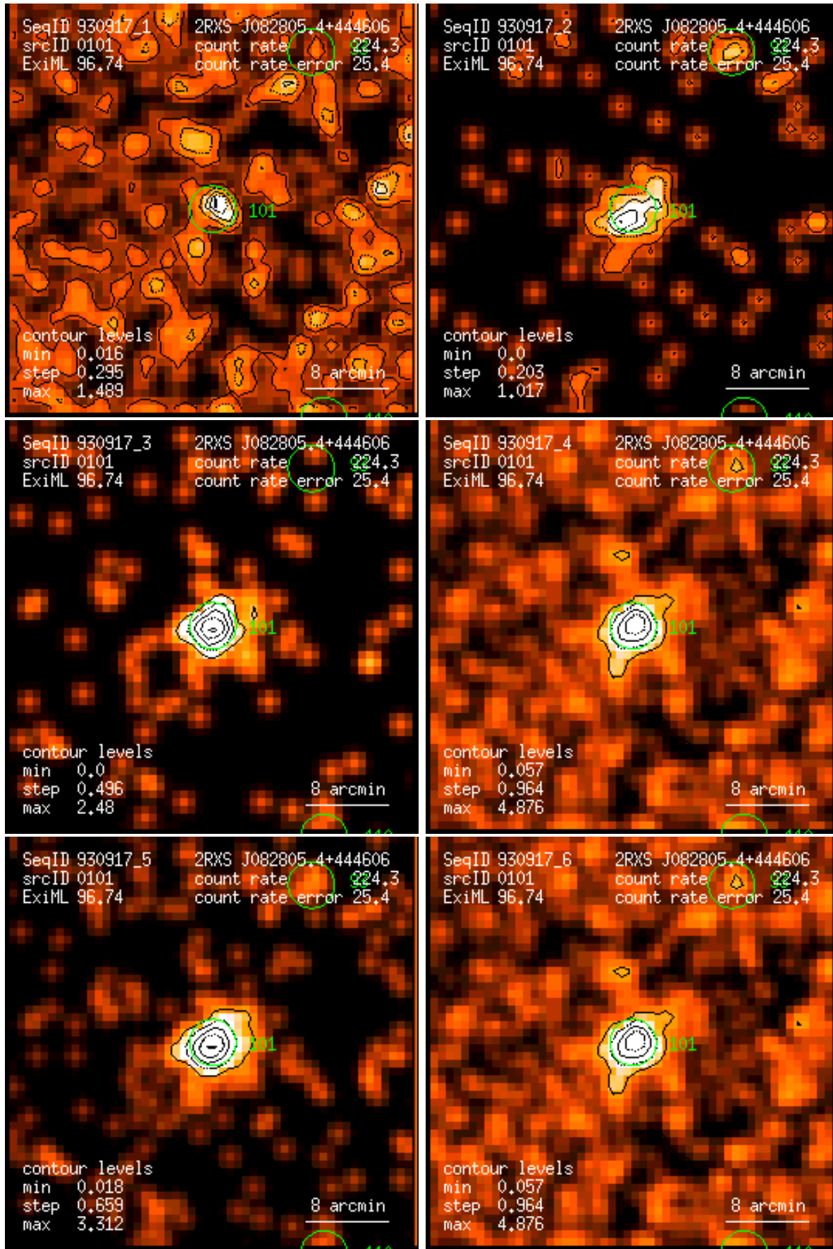
Figure 101: RASS 930917: detection 0101: band rate images, Gaussian filter: (1) PSPC channels 11 – 41, (2) 52 – 90, (3) 91 – 201, (4) 11 – 235, (5) 52 – 201, (6) 11 – 201. Broad band rates in counts/ks. Band rate contour levels in counts/ks/arcmin 2 .
