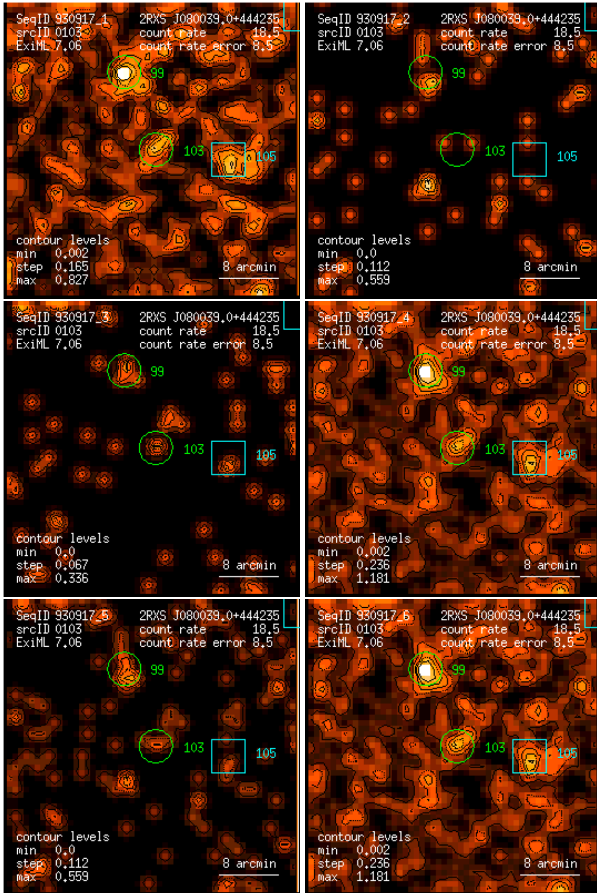
Figure 103: RASS 930917: detection 0103: band rate images, Gaussian filter: (1) PSPC channels 11 – 41, (2) 52 – 90, (3) 91 – 201, (4) 11 – 235, (5) 52 – 201, (6) 11 – 201. Broad band rates in counts/ks. Band rate contour levels in counts/ks/arcmin 2 .
