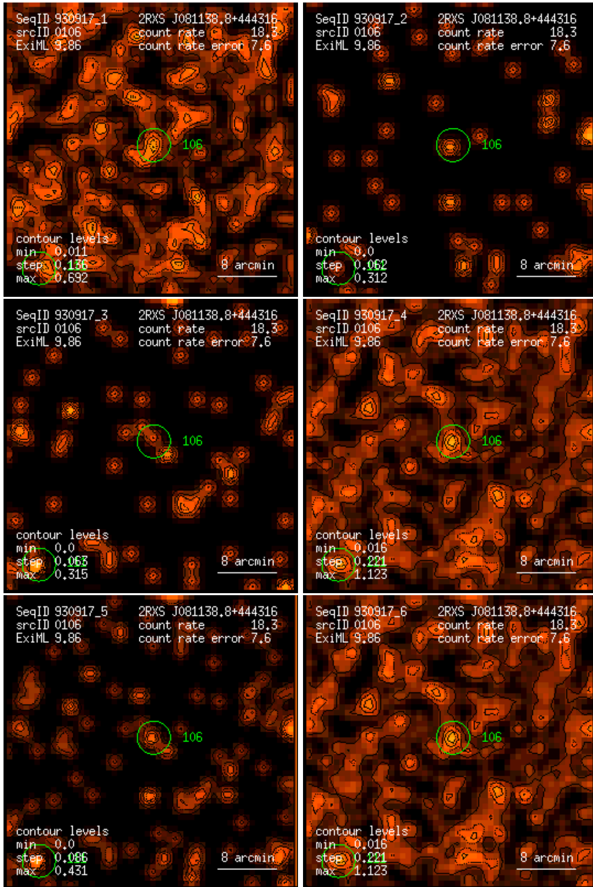
Figure 106: RASS 930917: detection 0106: band rate images, Gaussian filter: (1) PSPC channels 11 – 41, (2) 52 – 90, (3) 91 – 201, (4) 11 – 235, (5) 52 – 201, (6) 11 – 201. Broad band rates in counts/ks. Band rate contour levels in counts/ks/arcmin 2 .
