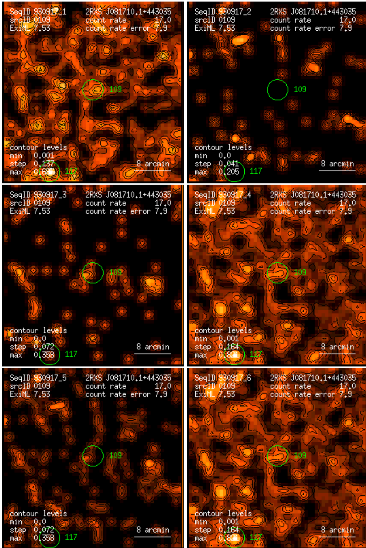
Figure 109: RASS 930917: detection 0109: band rate images, Gaussian filter: (1) PSPC channels 11 – 41, (2) 52 – 90, (3) 91 – 201, (4) 11 – 235, (5) 52 – 201, (6) 11 – 201. Broad band rates in counts/ks. Band rate contour levels in counts/ks/arcmin 2 .
