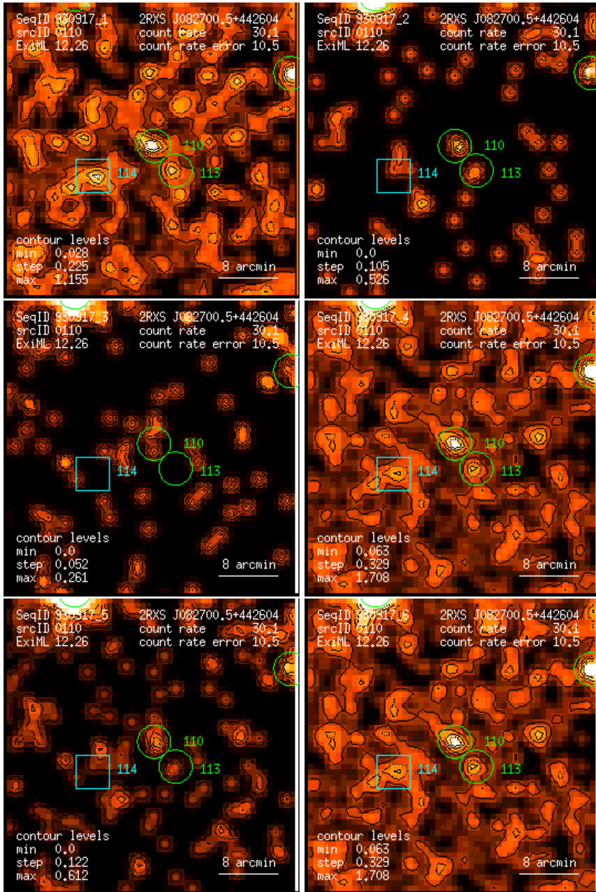
Figure 110: RASS 930917: detection 0110: band rate images, Gaussian filter: (1) PSPC channels 11 – 41, (2) 52 – 90, (3) 91 – 201, (4) 11 – 235, (5) 52 – 201, (6) 11 – 201. Broad band rates in counts/ks. Band rate contour levels in counts/ks/arcmin 2 .
