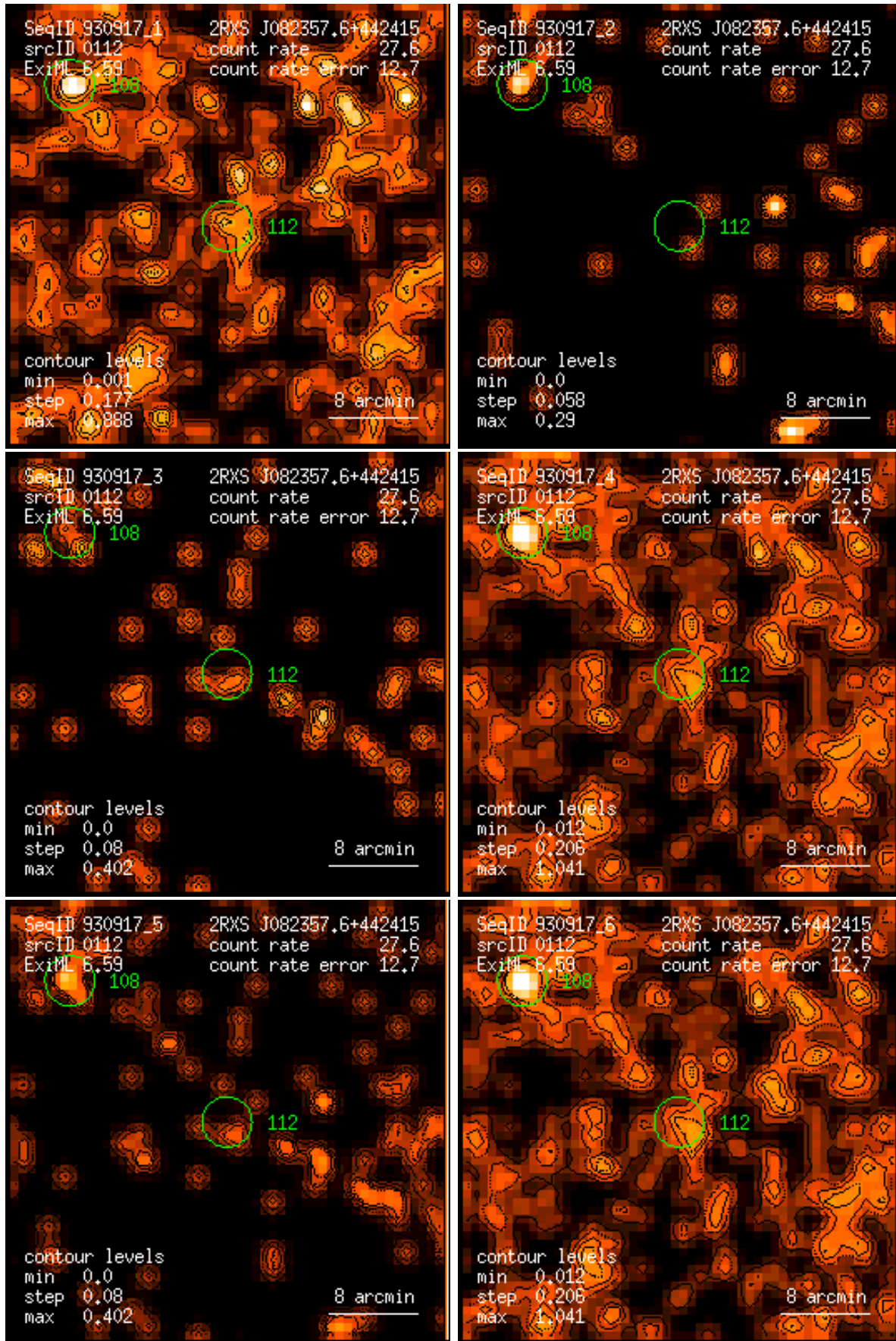
Figure 112: RASS 930917: detection 0112: band rate images, Gaussian filter: (1) PSPC channels 11 – 41, (2) 52 – 90, (3) 91 – 201, (4) 11 – 235, (5) 52 – 201, (6) 11 – 201. Broad band rates in counts/ks. Band rate contour levels in counts/ks/arcmin 2 .
