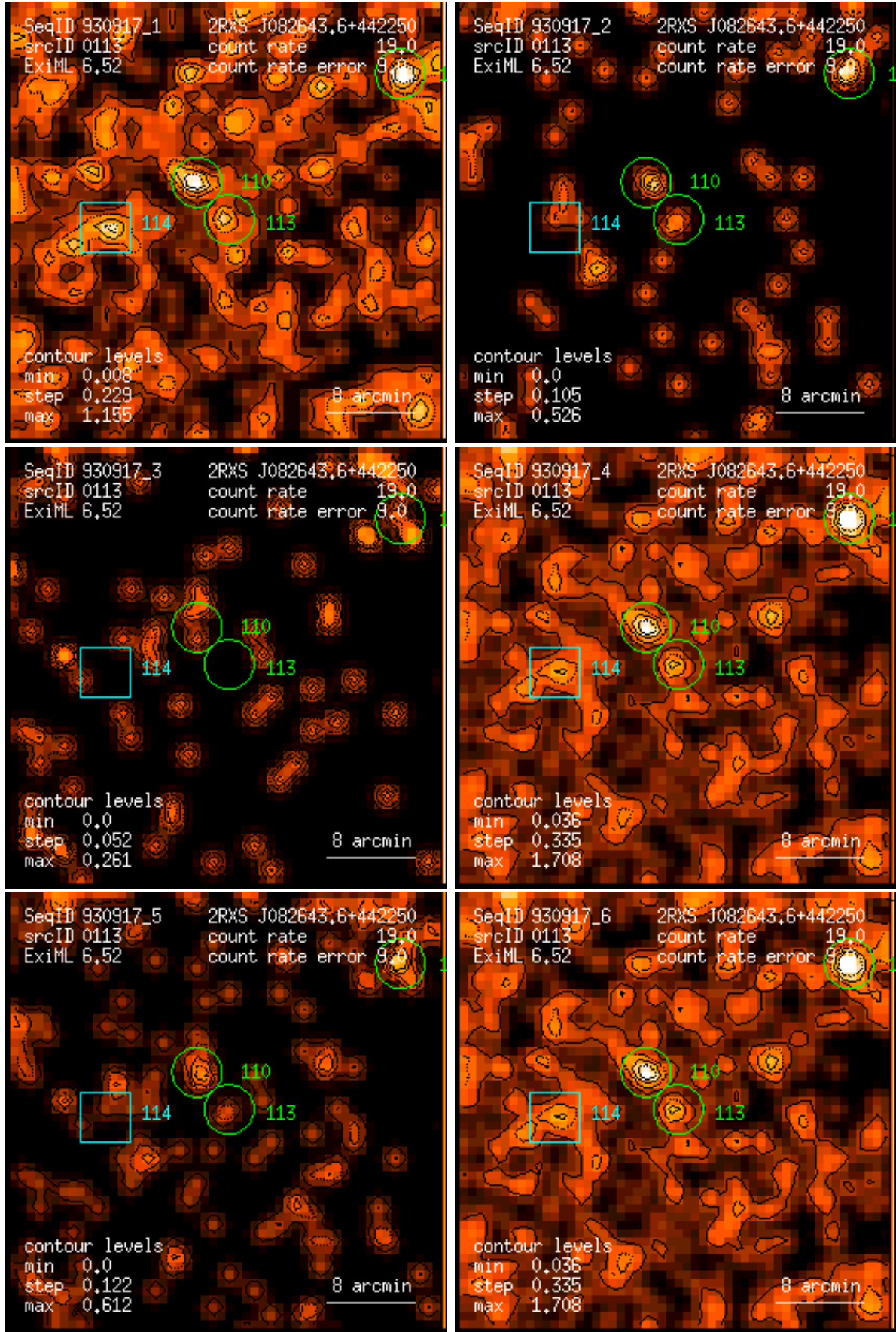
Figure 113: RASS 930917: detection 0113: band rate images, Gaussian filter: (1) PSPC channels 11 – 41, (2) 52 – 90, (3) 91 – 201, (4) 11 – 235, (5) 52 – 201, (6) 11 – 201. Broad band rates in counts/ks. Band rate contour levels in counts/ks/arcmin 2 .
