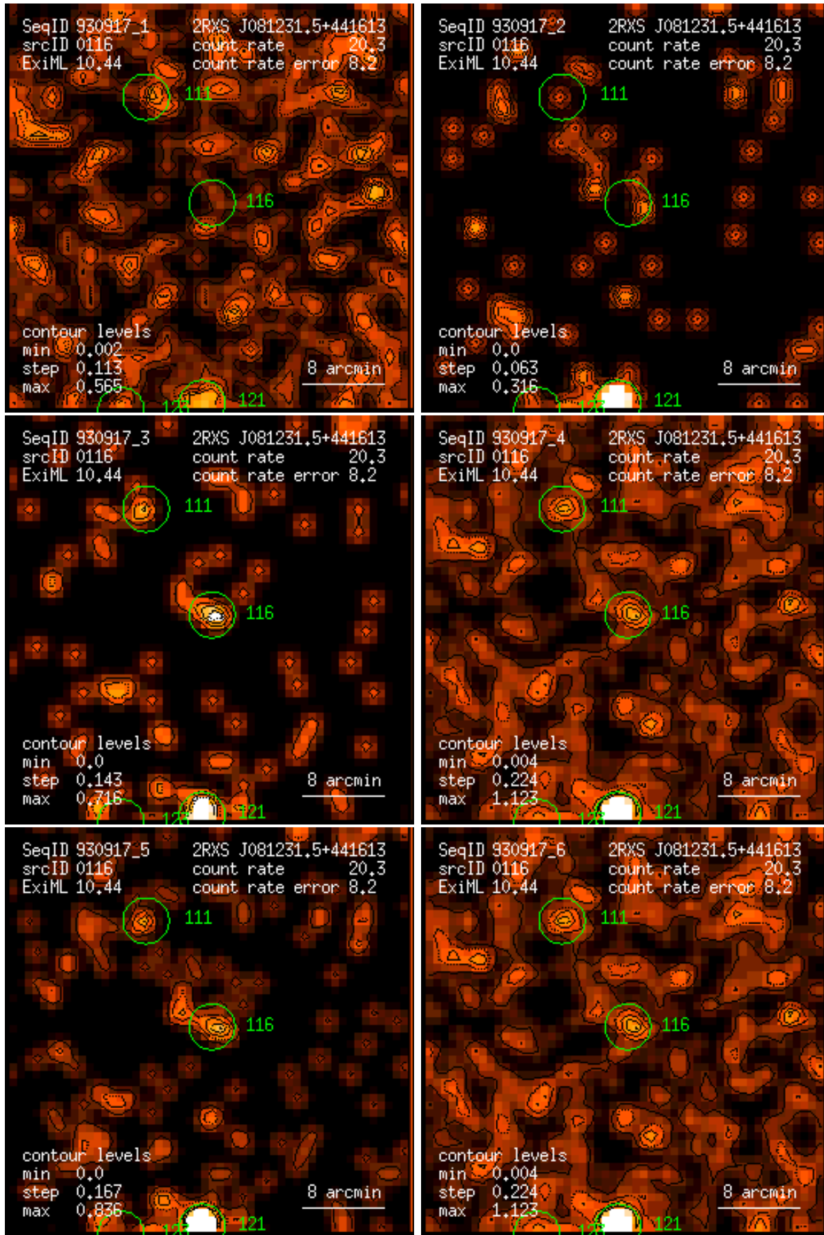
Figure 116: RASS 930917: detection 0116: band rate images, Gaussian filter: (1) PSPC channels 11 – 41, (2) 52 – 90, (3) 91 – 201, (4) 11 – 235, (5) 52 – 201, (6) 11 – 201. Broad band rates in counts/ks. Band rate contour levels in counts/ks/arcmin 2 .
