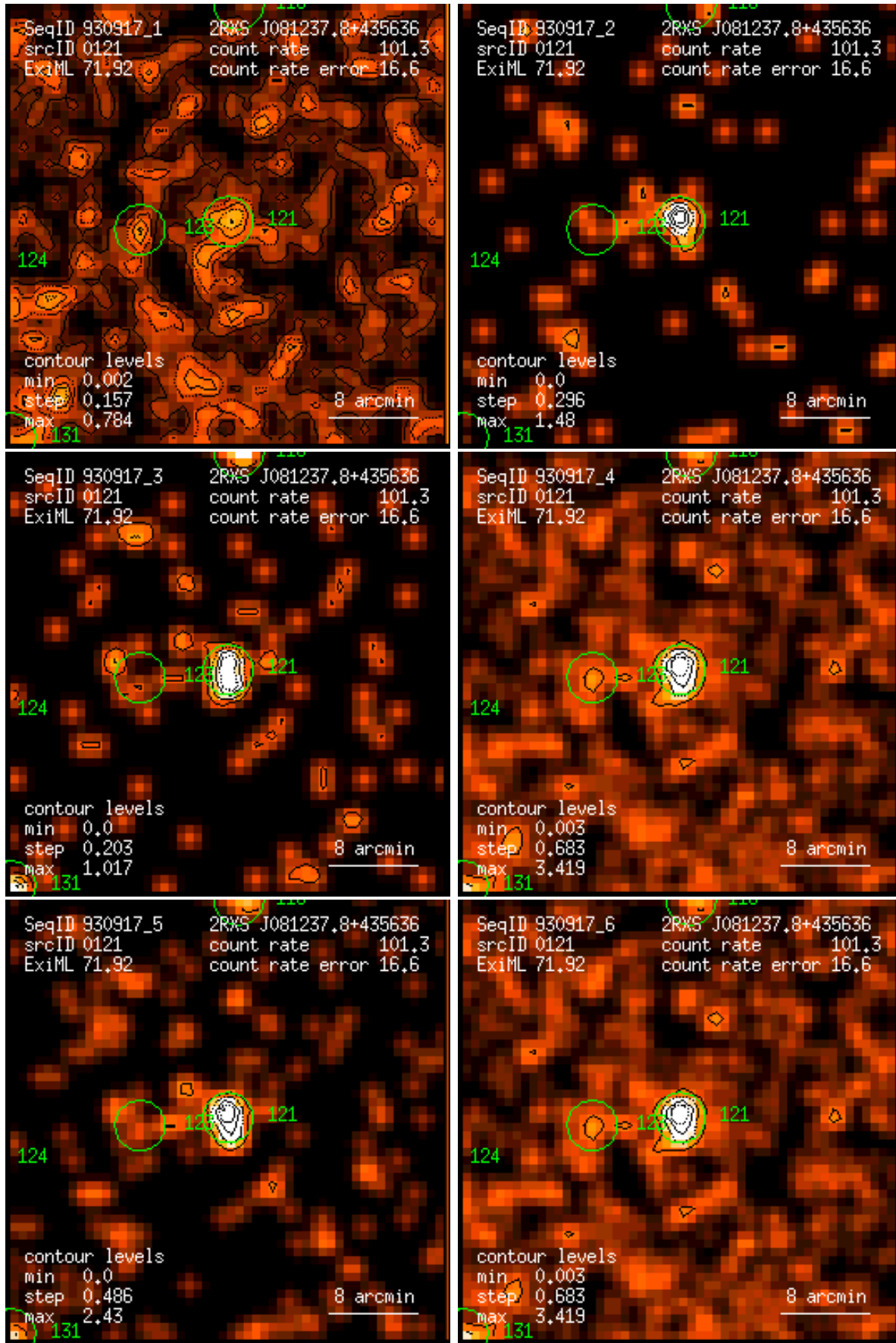
Figure 121: RASS 930917: detection 0121: band rate images, Gaussian filter: (1) PSPC channels 11 – 41, (2) 52 – 90, (3) 91 – 201, (4) 11 – 235, (5) 52 – 201, (6) 11 – 201. Broad band rates in counts/ks. Band rate contour levels in counts/ks/arcmin 2 .
