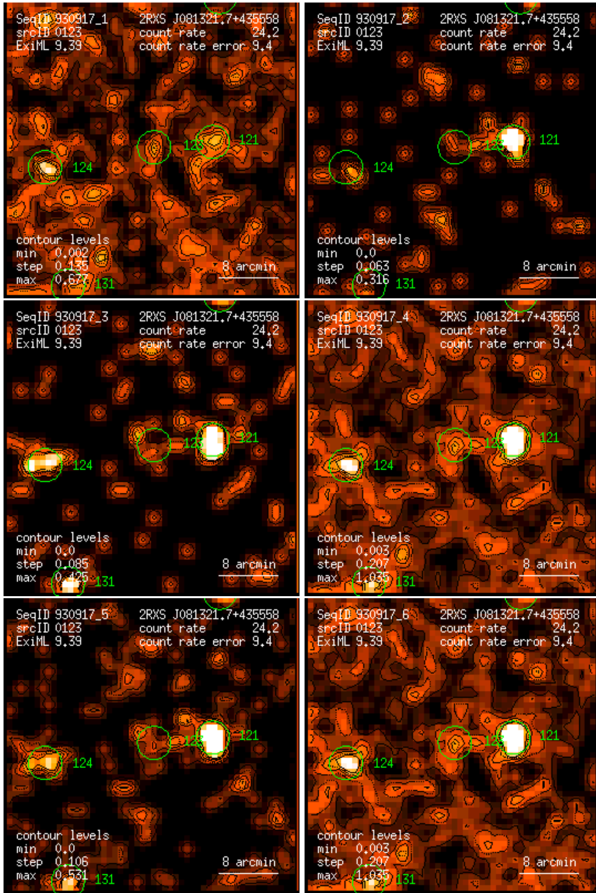
Figure 123: RASS 930917: detection 0123: band rate images, Gaussian filter: (1) PSPC channels 11 – 41, (2) 52 – 90, (3) 91 – 201, (4) 11 – 235, (5) 52 – 201, (6) 11 – 201. Broad band rates in counts/ks. Band rate contour levels in counts/ks/arcmin 2 .
