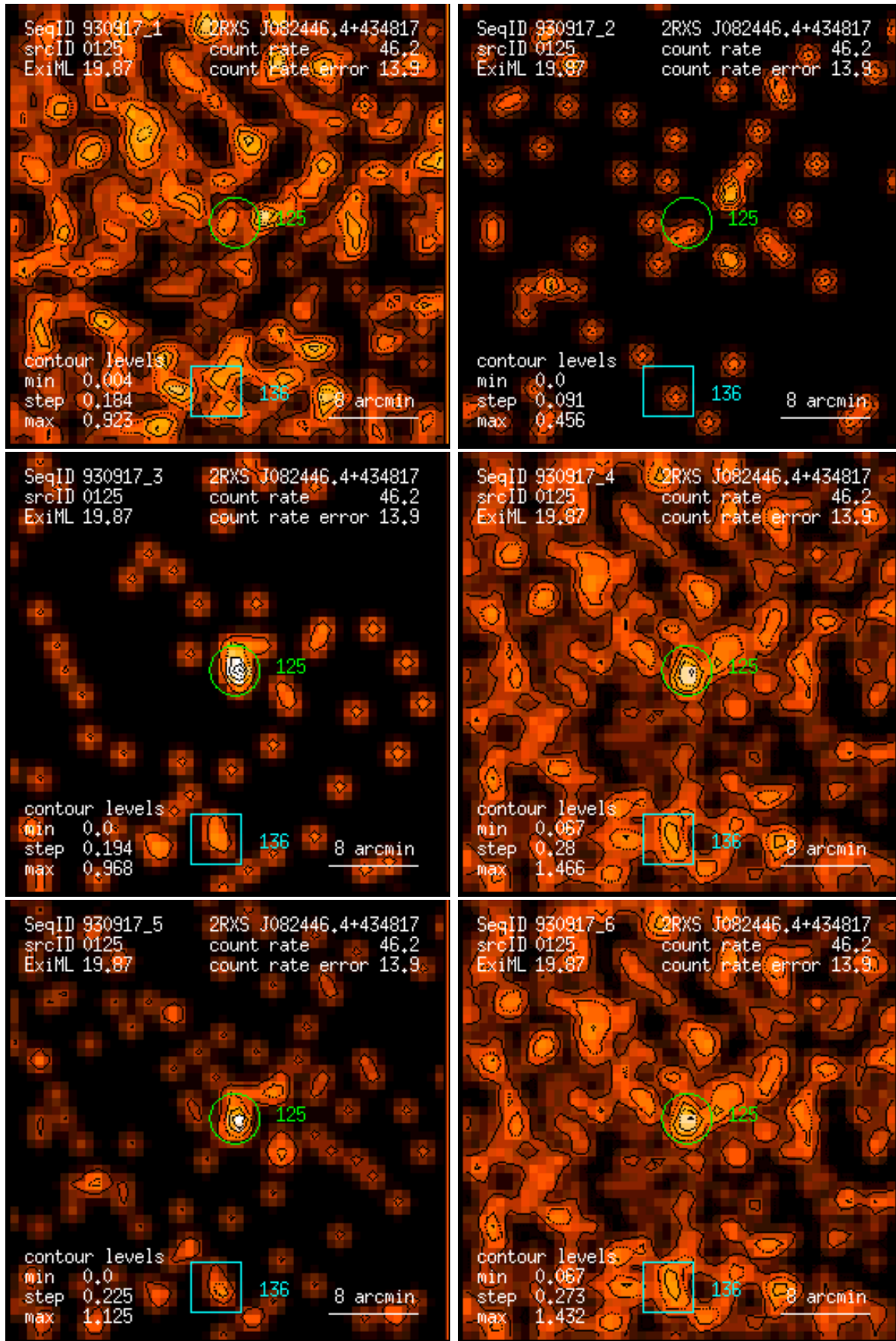
Figure 125: RASS 930917: detection 0125: band rate images, Gaussian filter: (1) PSPC channels 11 – 41, (2) 52 – 90, (3) 91 – 201, (4) 11 – 235, (5) 52 – 201, (6) 11 – 201. Broad band rates in counts/ks. Band rate contour levels in counts/ks/arcmin 2 .
