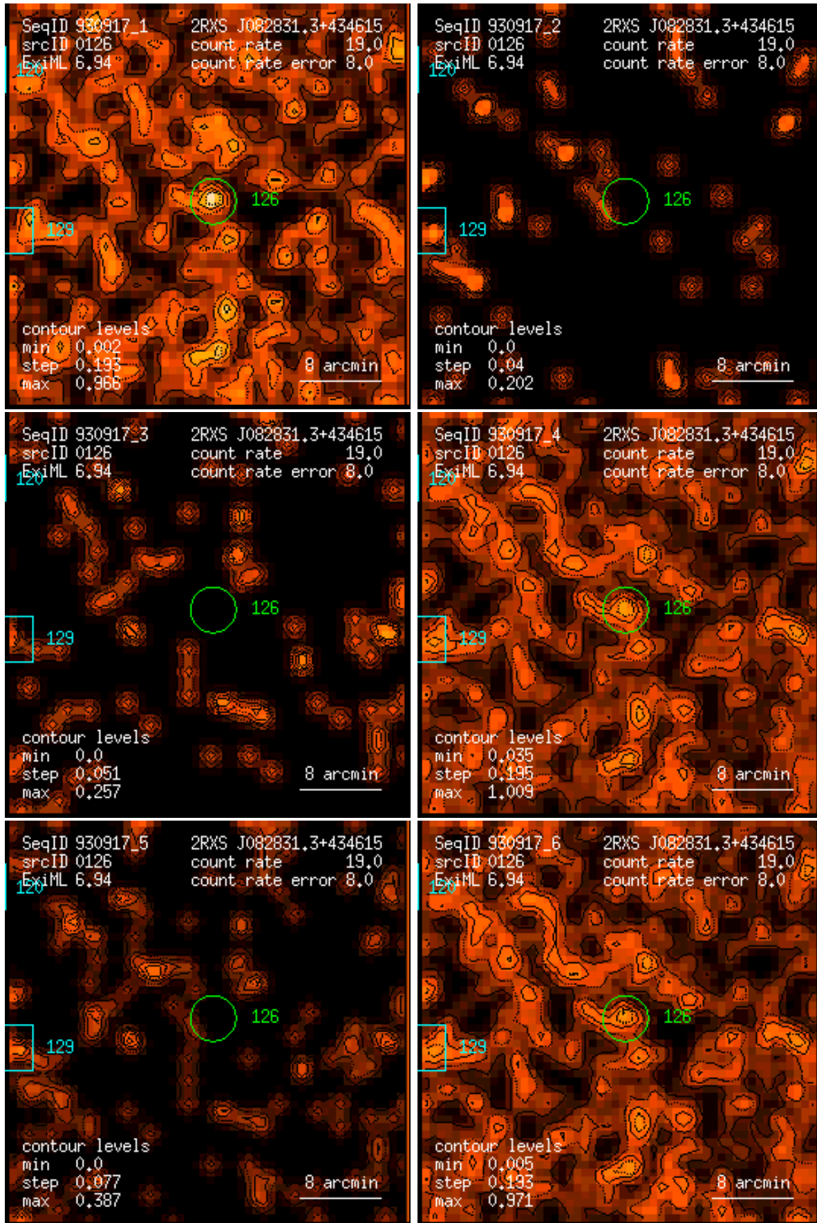
Figure 126: RASS 930917: detection 0126: band rate images, Gaussian filter: (1) PSPC channels 11 – 41, (2) 52 – 90, (3) 91 – 201, (4) 11 – 235, (5) 52 – 201, (6) 11 – 201. Broad band rates in counts/ks. Band rate contour levels in counts/ks/arcmin 2 .
