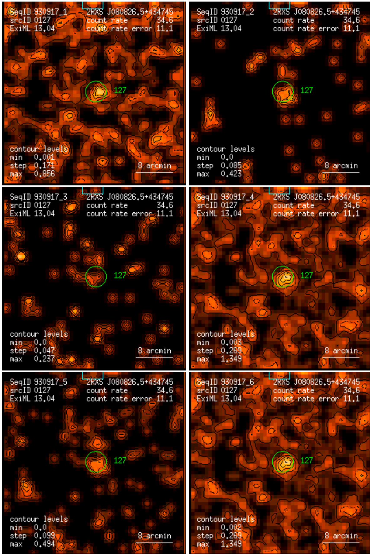
Figure 127: RASS 930917: detection 0127: band rate images, Gaussian filter: (1) PSPC channels 11 – 41, (2) 52 – 90, (3) 91 – 201, (4) 11 – 235, (5) 52 – 201, (6) 11 – 201. Broad band rates in counts/ks. Band rate contour levels in counts/ks/arcmin 2 .
