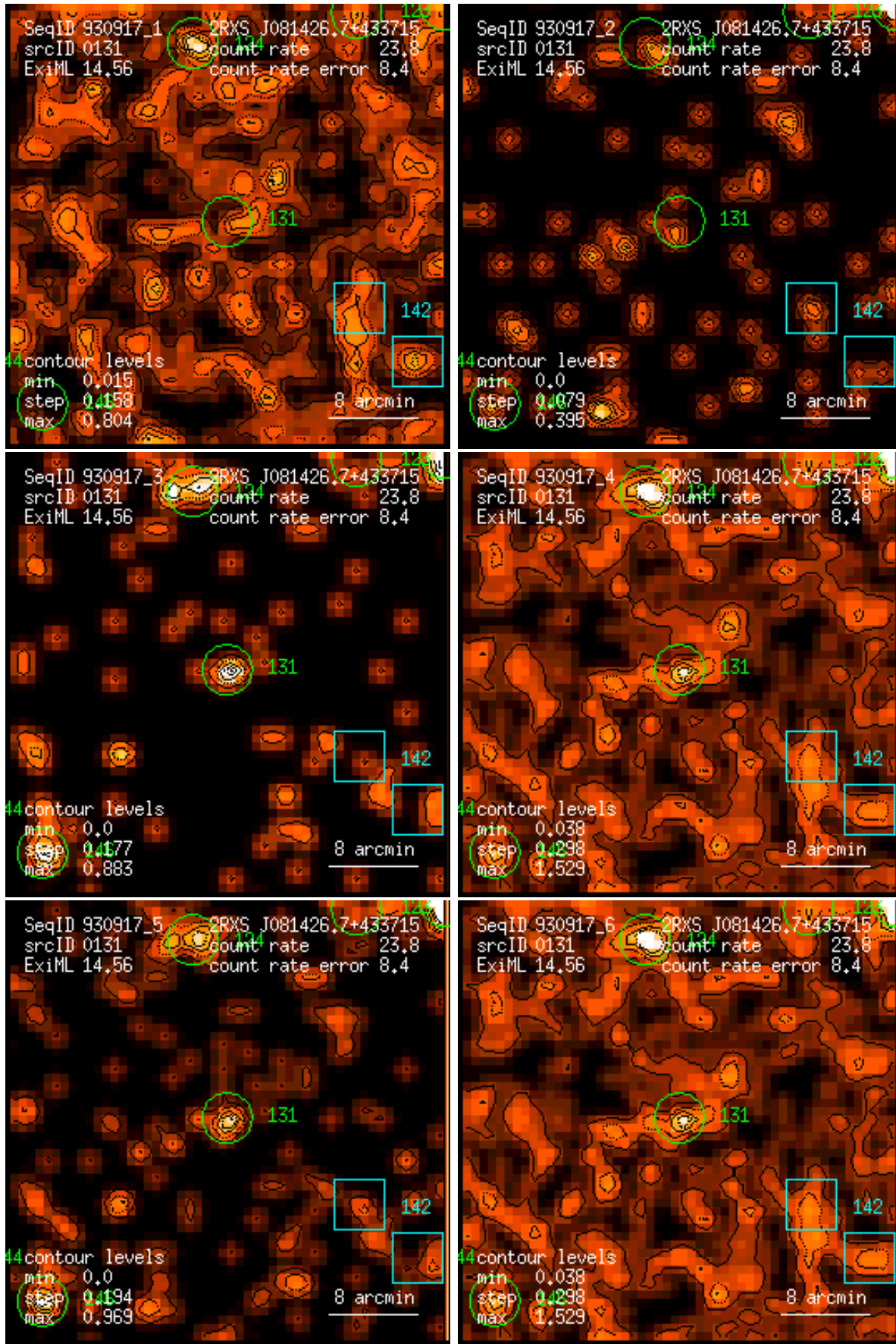
Figure 131: RASS 930917: detection 0131: band rate images, Gaussian filter: (1) PSPC channels 11 – 41, (2) 52 – 90, (3) 91 – 201, (4) 11 – 235, (5) 52 – 201, (6) 11 – 201. Broad band rates in counts/ks. Band rate contour levels in counts/ks/arcmin 2 .
