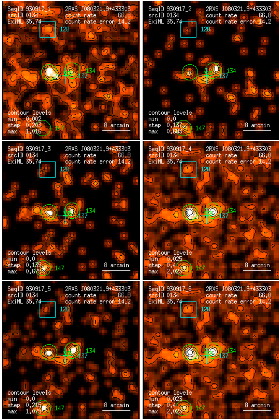
Figure 134: RASS 930917: detection 0134: band rate images, Gaussian filter: (1) PSPC channels 11 – 41, (2) 52 – 90, (3) 91 – 201, (4) 11 – 235, (5) 52 – 201, (6) 11 – 201. Broad band rates in counts/ks. Band rate contour levels in counts/ks/arcmin 2 .
