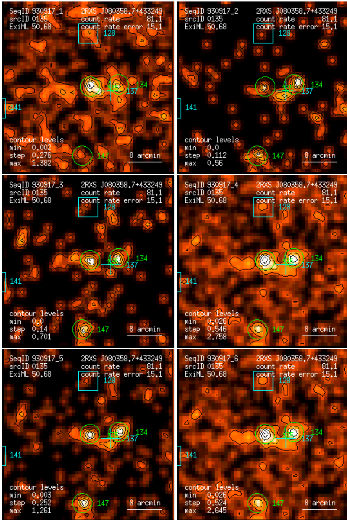
Figure 135: RASS 930917: detection 0135: band rate images, Gaussian filter: (1) PSPC channels 11 – 41, (2) 52 – 90, (3) 91 – 201, (4) 11 – 235, (5) 52 – 201, (6) 11 – 201. Broad band rates in counts/ks. Band rate contour levels in counts/ks/arcmin 2 .
