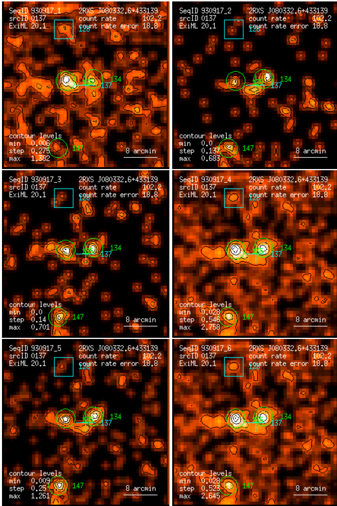
Figure 137: RASS 930917: detection 0137: band rate images, Gaussian filter: (1) PSPC channels 11 – 41, (2) 52 – 90, (3) 91 – 201, (4) 11 – 235, (5) 52 – 201, (6) 11 – 201. Broad band rates in counts/ks. Band rate contour levels in counts/ks/arcmin 2 .
