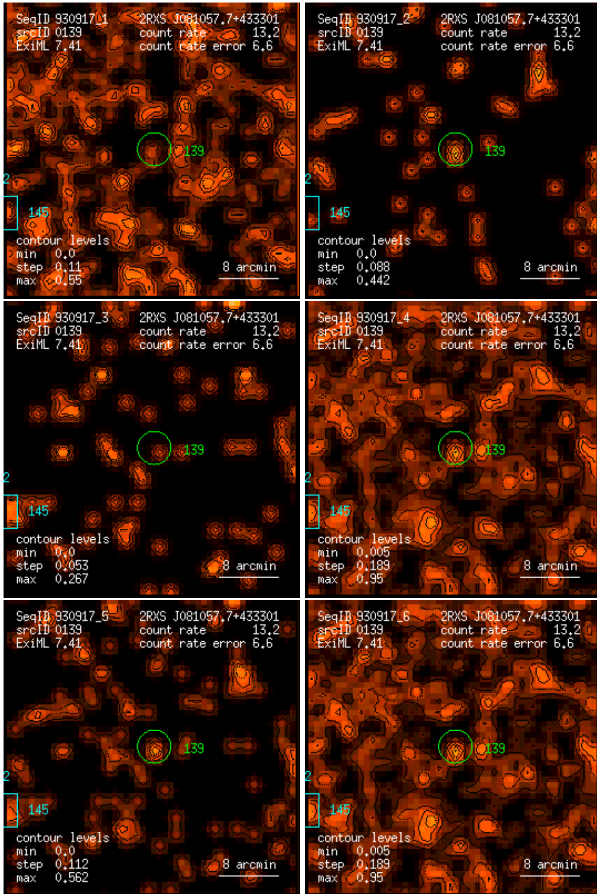
Figure 139: RASS 930917: detection 0139: band rate images, Gaussian filter: (1) PSPC channels 11 – 41, (2) 52 – 90, (3) 91 – 201, (4) 11 – 235, (5) 52 – 201, (6) 11 – 201. Broad band rates in counts/ks. Band rate contour levels in counts/ks/arcmin 2 .
