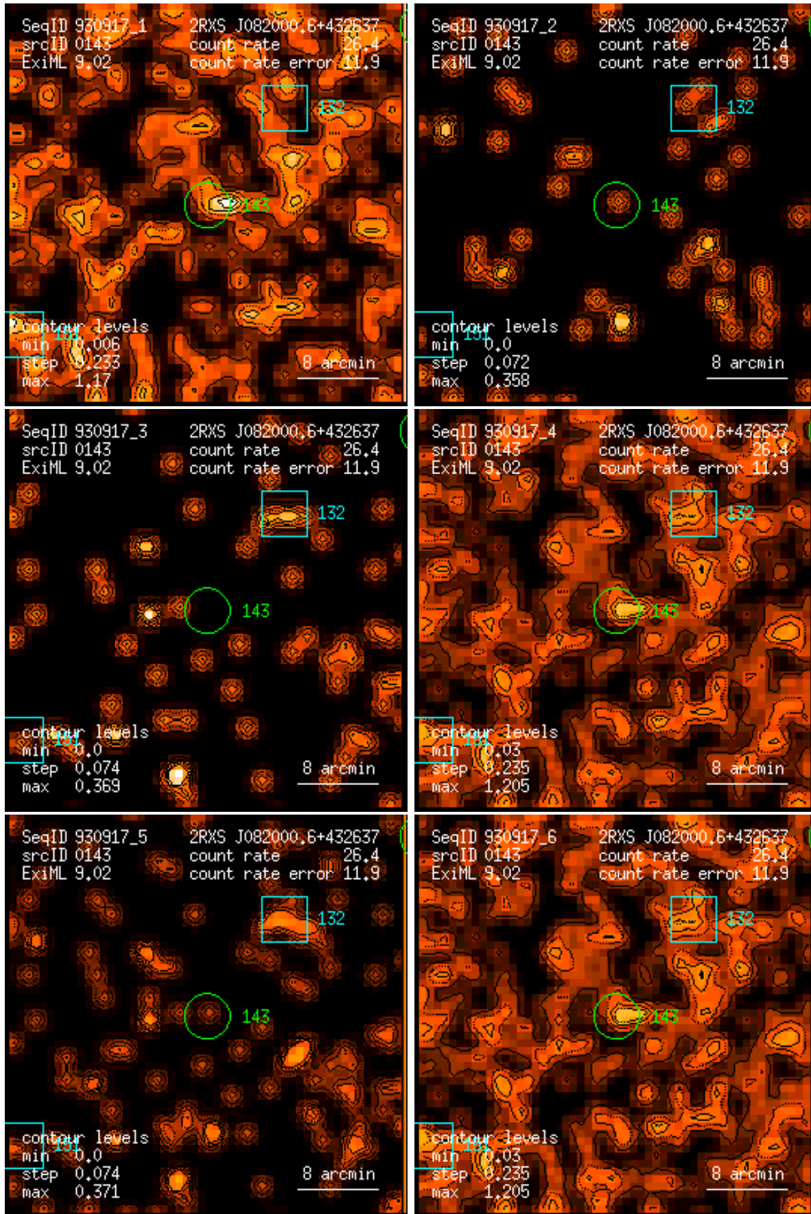
Figure 143: RASS 930917: detection 0143: band rate images, Gaussian filter: (1) PSPC channels 11 – 41, (2) 52 – 90, (3) 91 – 201, (4) 11 – 235, (5) 52 – 201, (6) 11 – 201. Broad band rates in counts/ks. Band rate contour levels in counts/ks/arcmin 2 .
