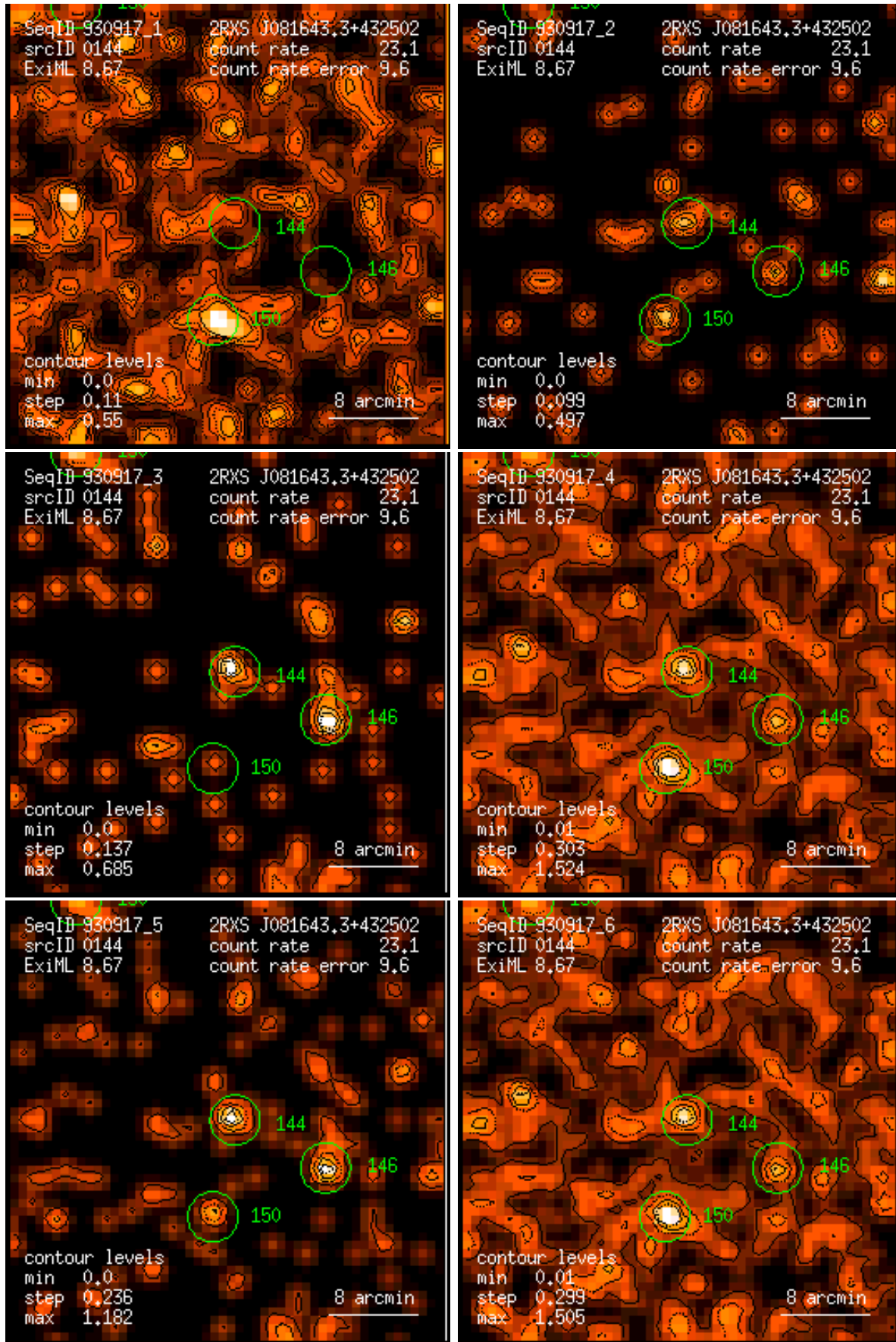
Figure 144: RASS 930917: detection 0144: band rate images, Gaussian filter: (1) PSPC channels 11 – 41, (2) 52 – 90, (3) 91 – 201, (4) 11 – 235, (5) 52 – 201, (6) 11 – 201. Broad band rates in counts/ks. Band rate contour levels in counts/ks/arcmin 2 .
