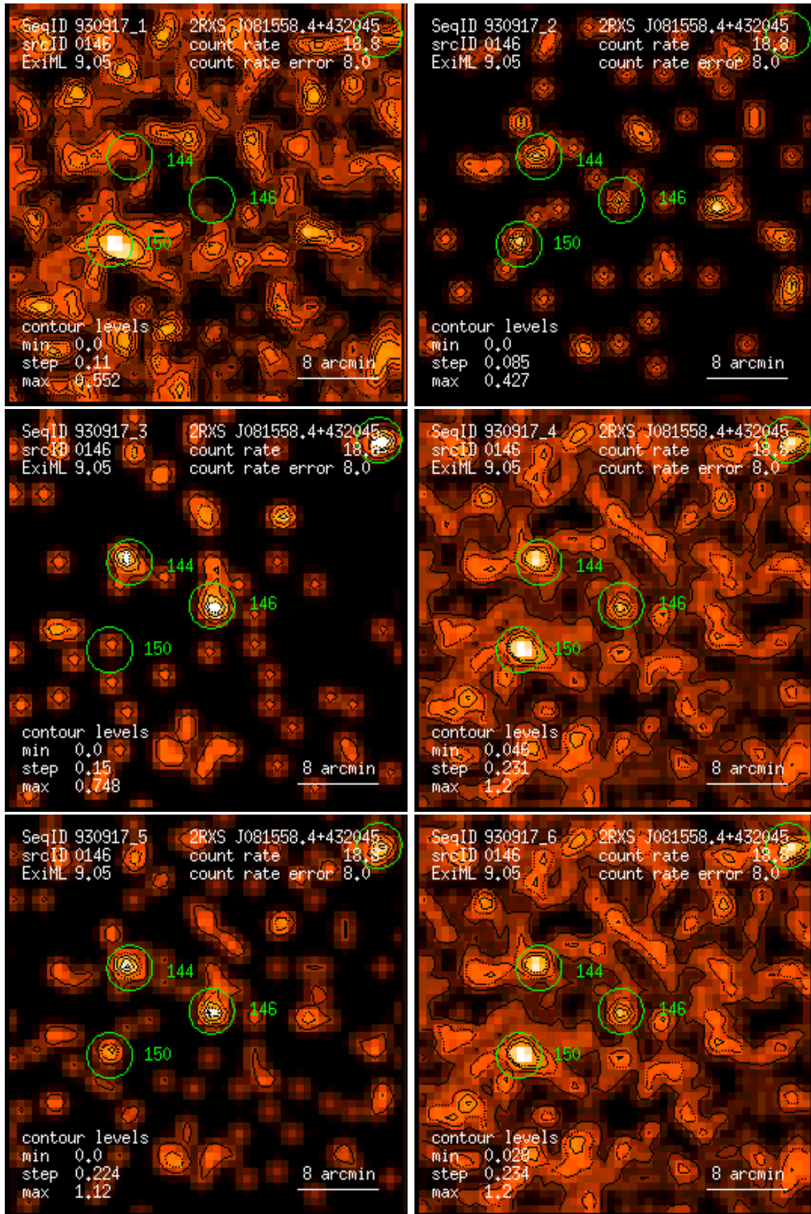
Figure 146: RASS 930917: detection 0146: band rate images, Gaussian filter: (1) PSPC channels 11 – 41, (2) 52 – 90, (3) 91 – 201, (4) 11 – 235, (5) 52 – 201, (6) 11 – 201. Broad band rates in counts/ks. Band rate contour levels in counts/ks/arcmin 2 .
