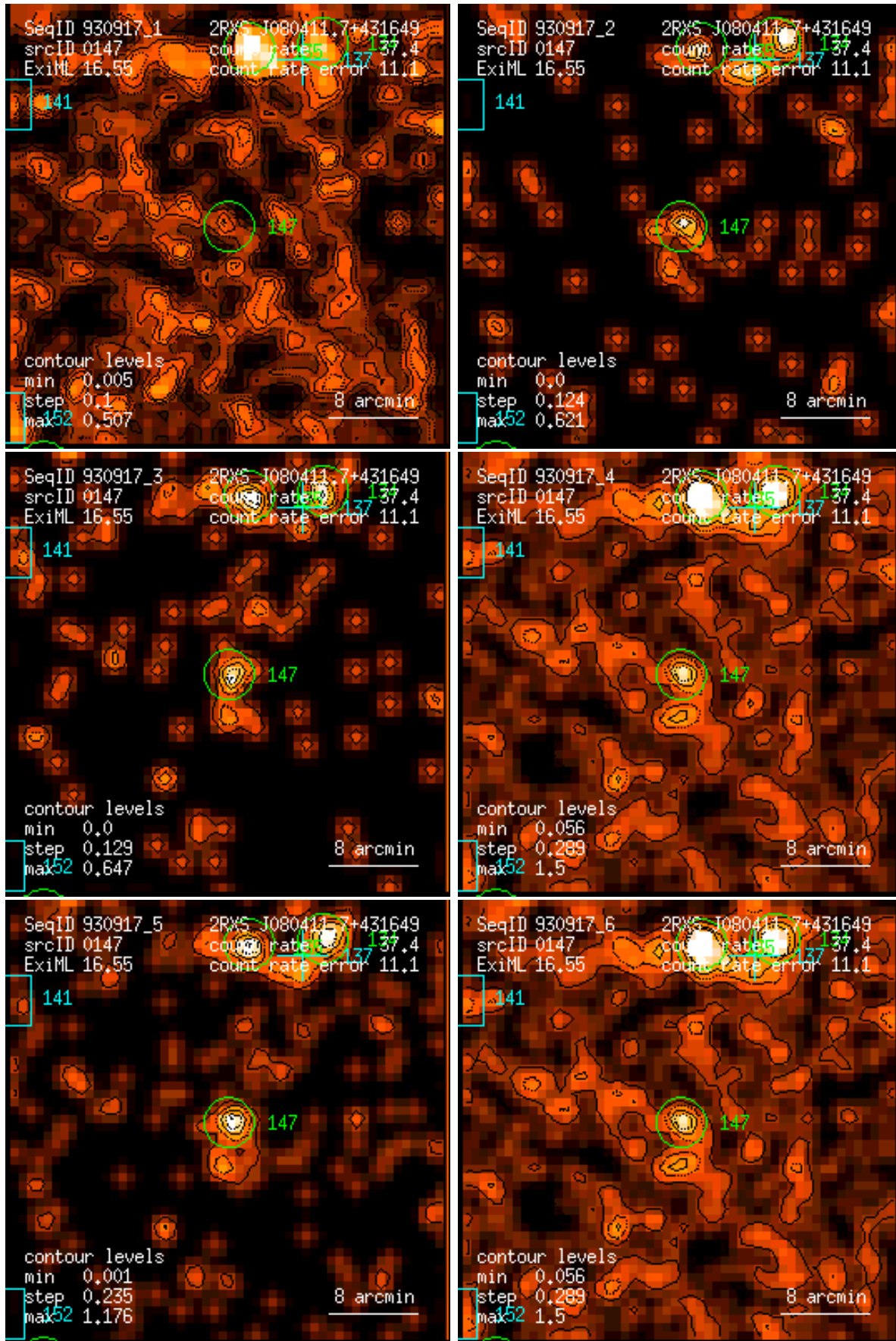
Figure 147: RASS 930917: detection 0147: band rate images, Gaussian filter: (1) PSPC channels 11 – 41, (2) 52 – 90, (3) 91 – 201, (4) 11 – 235, (5) 52 – 201, (6) 11 – 201. Broad band rates in counts/ks. Band rate contour levels in counts/ks/arcmin 2 .
