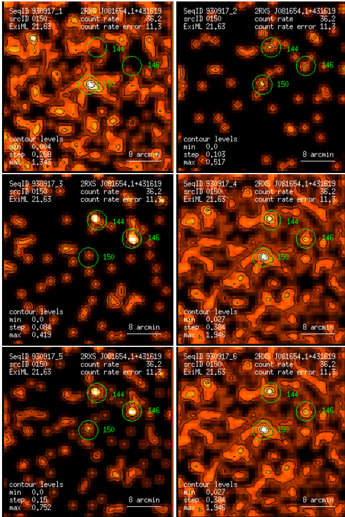
Figure 150: RASS 930917: detection 0150: band rate images, Gaussian filter: (1) PSPC channels 11 – 41, (2) 52 – 90, (3) 91 – 201, (4) 11 – 235, (5) 52 – 201, (6) 11 – 201. Broad band rates in counts/ks. Band rate contour levels in counts/ks/arcmin 2 .
