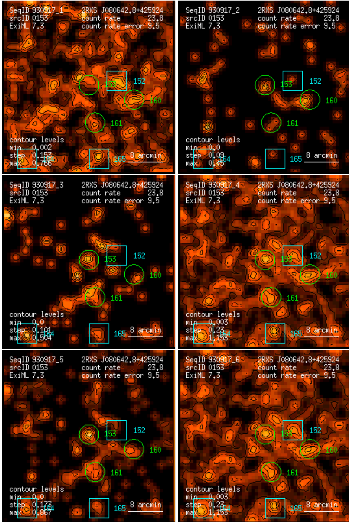
Figure 153: RASS 930917: detection 0153: band rate images, Gaussian filter: (1) PSPC channels 11 – 41, (2) 52 – 90, (3) 91 – 201, (4) 11 – 235, (5) 52 – 201, (6) 11 – 201. Broad band rates in counts/ks. Band rate contour levels in counts/ks/arcmin 2 .
