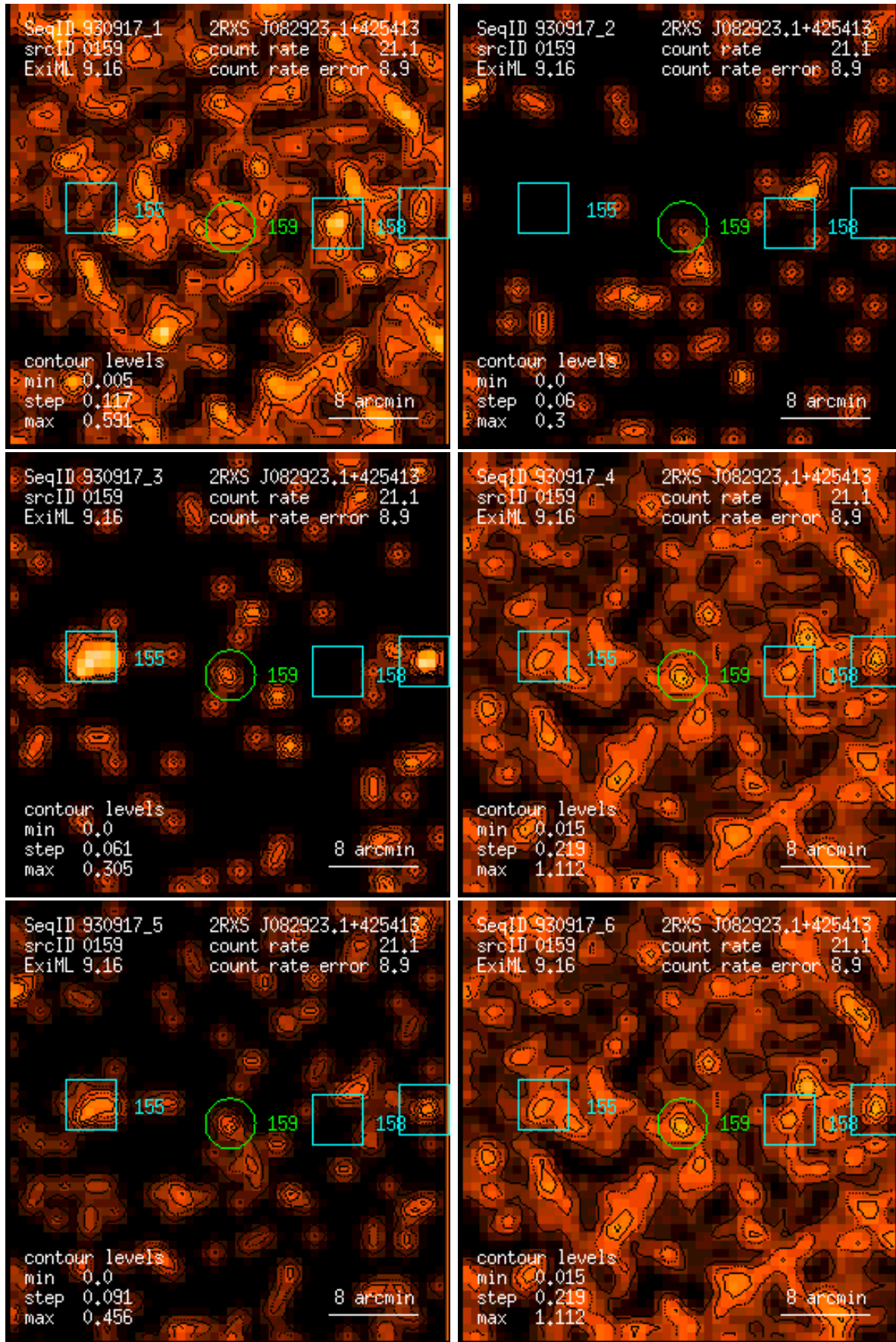
Figure 159: RASS 930917: detection 0159: band rate images, Gaussian filter: (1) PSPC channels 11 – 41, (2) 52 – 90, (3) 91 – 201, (4) 11 – 235, (5) 52 – 201, (6) 11 – 201. Broad band rates in counts/ks. Band rate contour levels in counts/ks/arcmin 2 .
