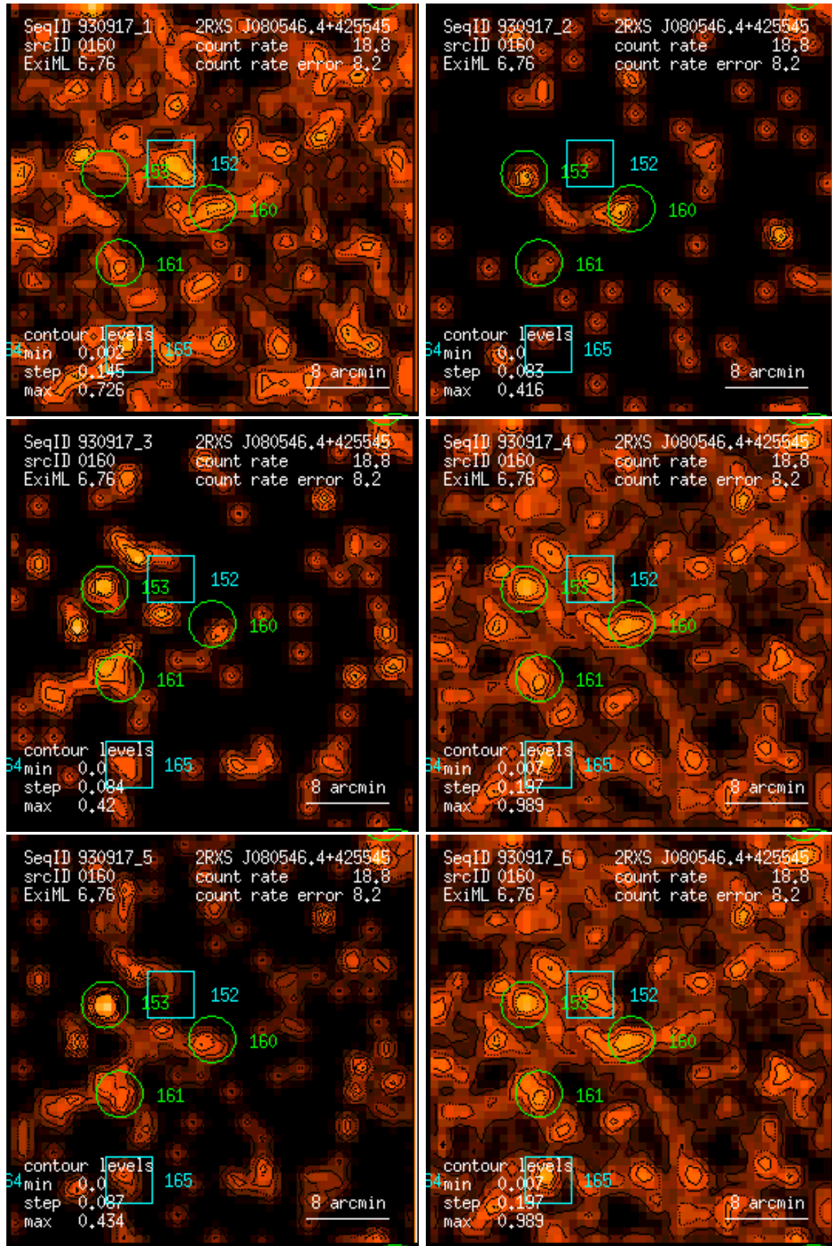
Figure 160: RASS 930917: detection 0160: band rate images, Gaussian filter: (1) PSPC channels 11 – 41, (2) 52 – 90, (3) 91 – 201, (4) 11 – 235, (5) 52 – 201, (6) 11 – 201. Broad band rates in counts/ks. Band rate contour levels in counts/ks/arcmin 2 .
