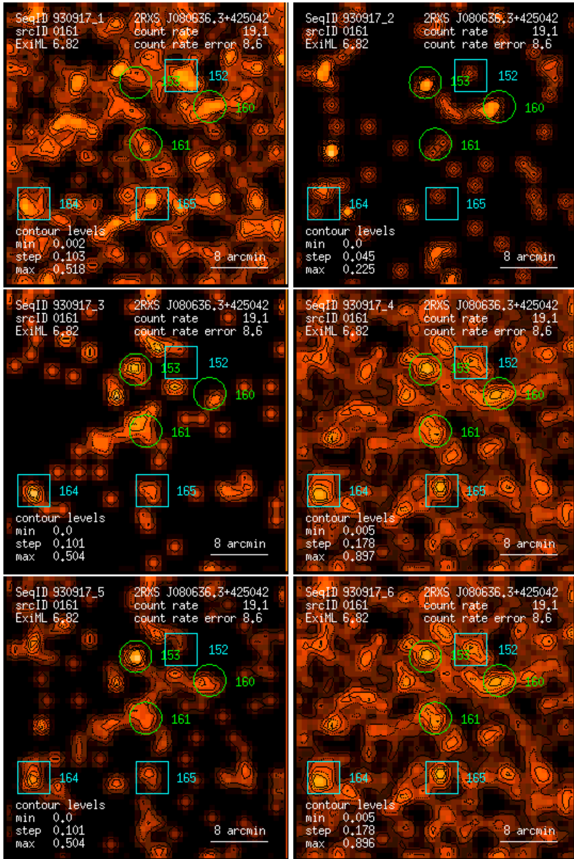
Figure 161: RASS 930917: detection 0161: band rate images, Gaussian filter: (1) PSPC channels 11 – 41, (2) 52 – 90, (3) 91 – 201, (4) 11 – 235, (5) 52 – 201, (6) 11 – 201. Broad band rates in counts/ks. Band rate contour levels in counts/ks/arcmin 2 .
