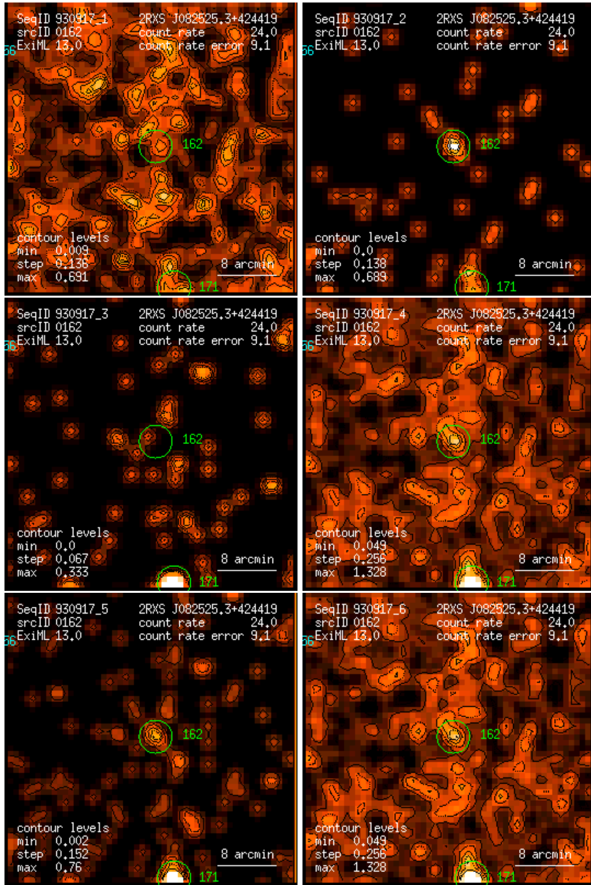
Figure 162: RASS 930917: detection 0162: band rate images, Gaussian filter: (1) PSPC channels 11 – 41, (2) 52 – 90, (3) 91 – 201, (4) 11 – 235, (5) 52 – 201, (6) 11 – 201. Broad band rates in counts/ks. Band rate contour levels in counts/ks/arcmin 2 .
