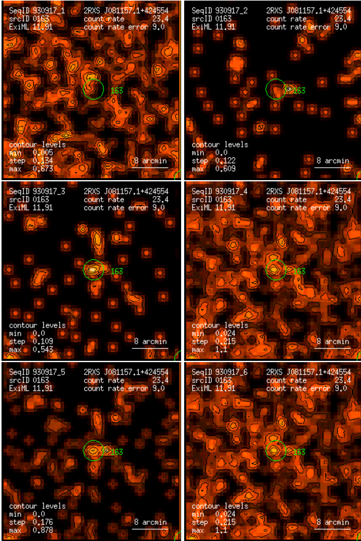
Figure 163: RASS 930917: detection 0163: band rate images, Gaussian filter: (1) PSPC channels 11 – 41, (2) 52 – 90, (3) 91 – 201, (4) 11 – 235, (5) 52 – 201, (6) 11 – 201. Broad band rates in counts/ks. Band rate contour levels in counts/ks/arcmin 2 .
