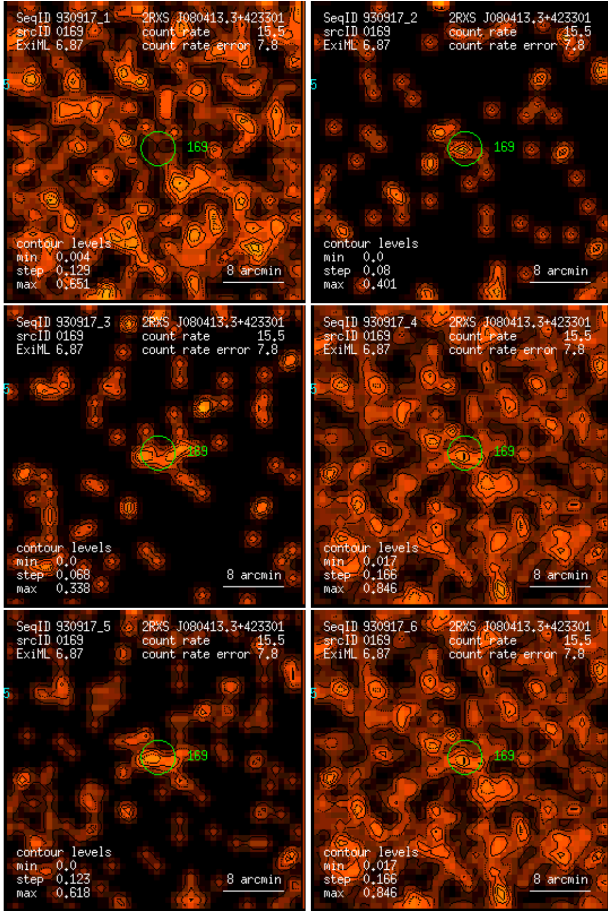
Figure 169: RASS 930917: detection 0169: band rate images, Gaussian filter: (1) PSPC channels 11 – 41, (2) 52 – 90, (3) 91 – 201, (4) 11 – 235, (5) 52 – 201, (6) 11 – 201. Broad band rates in counts/ks. Band rate contour levels in counts/ks/arcmin 2 .
