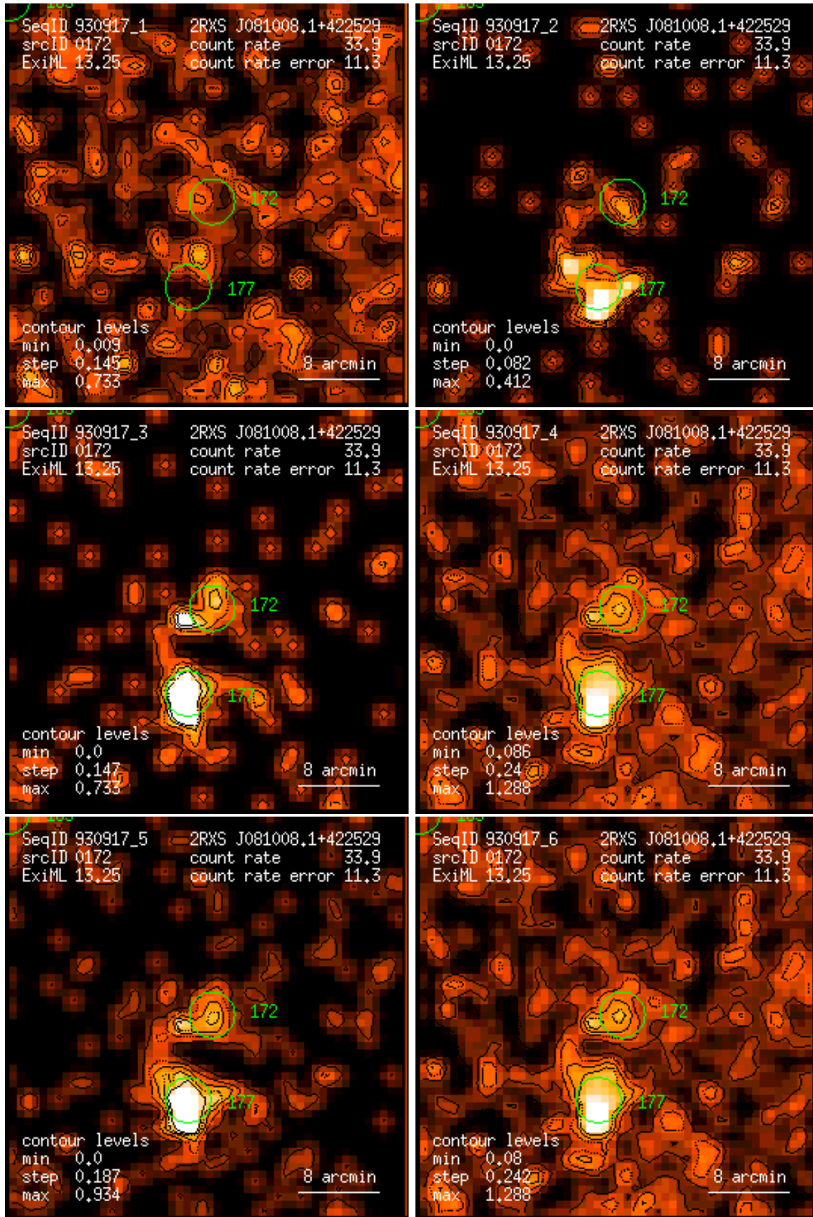
Figure 172: RASS 930917: detection 0172: band rate images, Gaussian filter: (1) PSPC channels 11 – 41, (2) 52 – 90, (3) 91 – 201, (4) 11 – 235, (5) 52 – 201, (6) 11 – 201. Broad band rates in counts/ks. Band rate contour levels in counts/ks/arcmin 2 .
