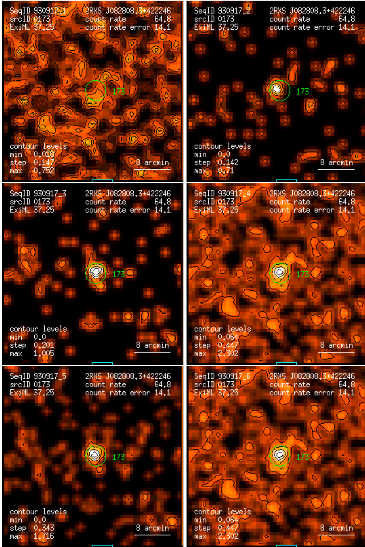
Figure 173: RASS 930917: detection 0173: band rate images, Gaussian filter: (1) PSPC channels 11 – 41, (2) 52 – 90, (3) 91 – 201, (4) 11 – 235, (5) 52 – 201, (6) 11 – 201. Broad band rates in counts/ks. Band rate contour levels in counts/ks/arcmin 2 .
