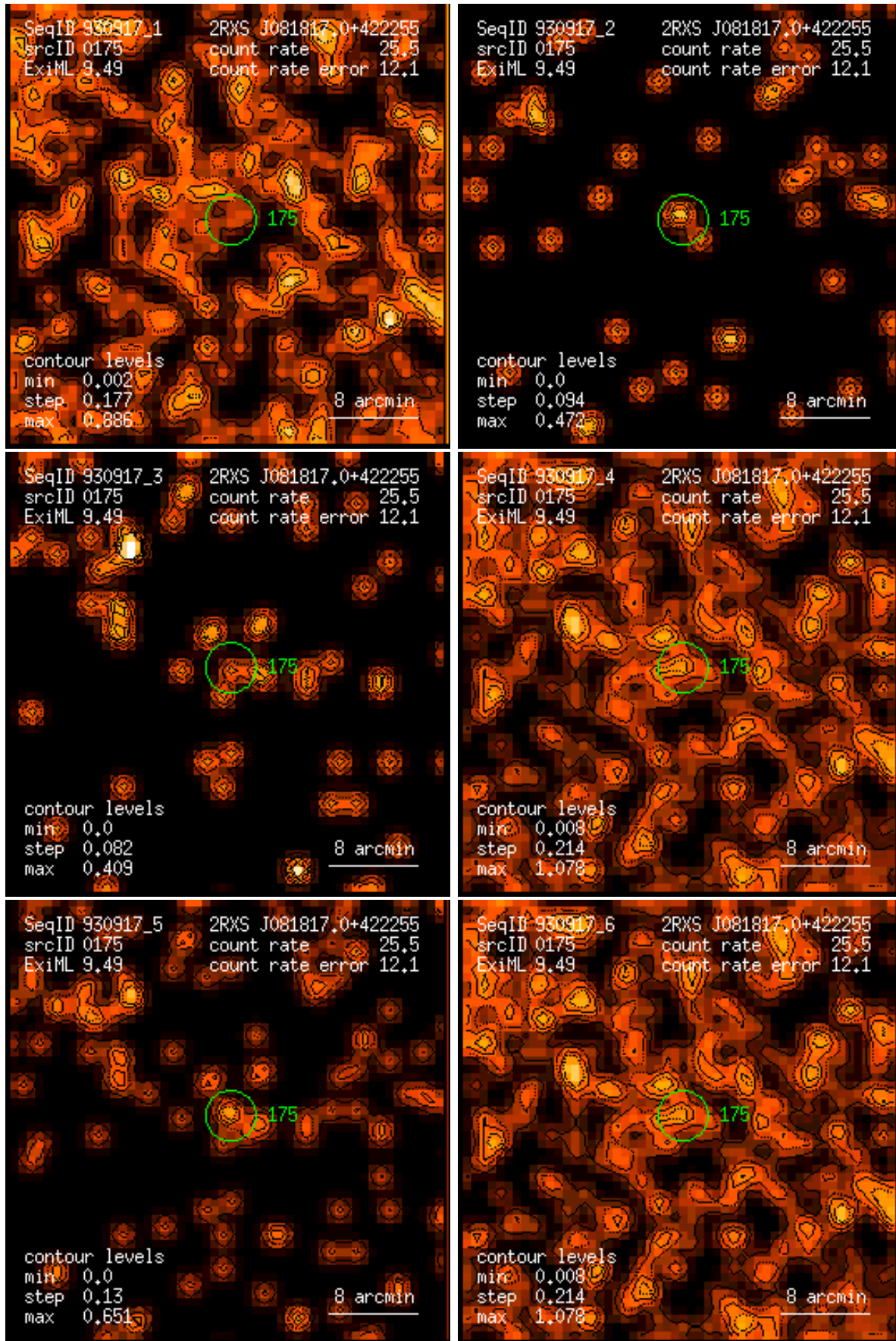
Figure 175: RASS 930917: detection 0175: band rate images, Gaussian filter: (1) PSPC channels 11 – 41, (2) 52 – 90, (3) 91 – 201, (4) 11 – 235, (5) 52 – 201, (6) 11 – 201. Broad band rates in counts/ks. Band rate contour levels in counts/ks/arcmin 2 .
