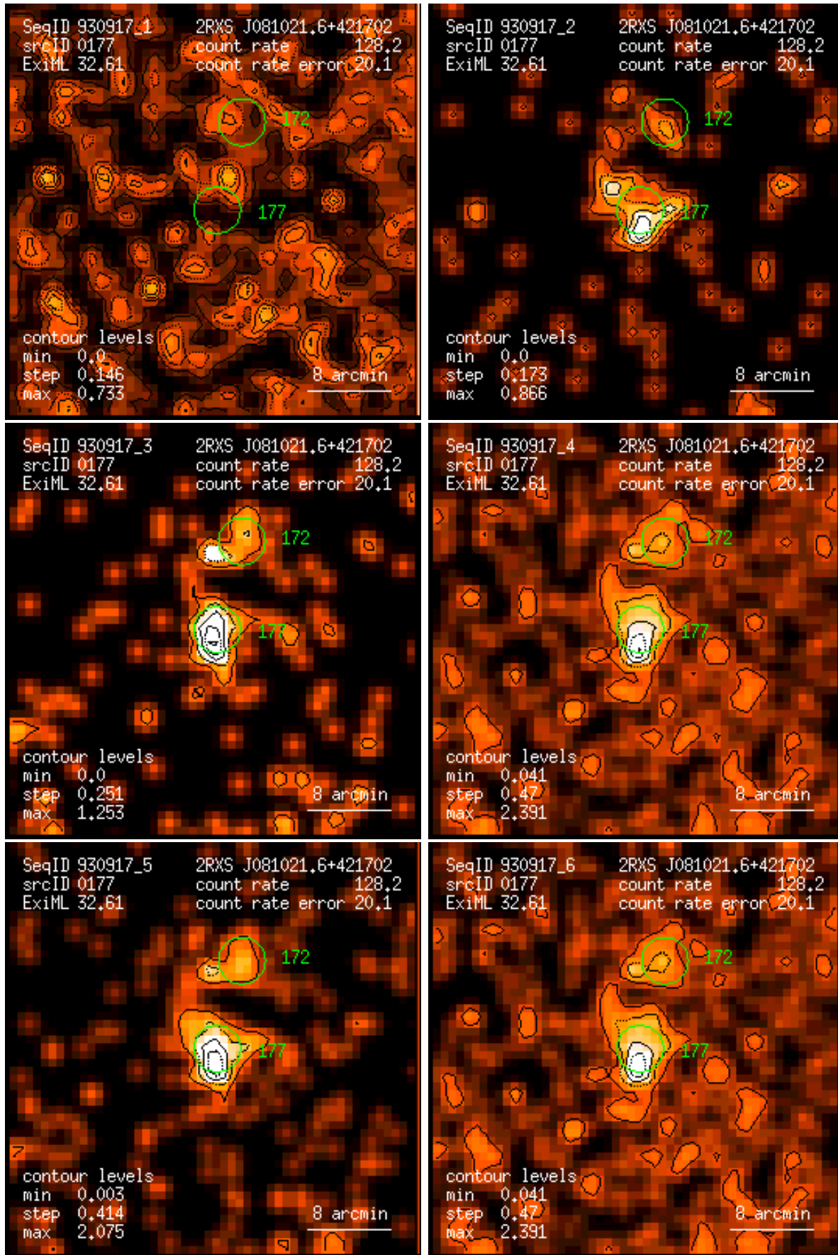
Figure 177: RASS 930917: detection 0177: band rate images, Gaussian filter: (1) PSPC channels 11 – 41, (2) 52 – 90, (3) 91 – 201, (4) 11 – 235, (5) 52 – 201, (6) 11 – 201. Broad band rates in counts/ks. Band rate contour levels in counts/ks/arcmin 2 .
