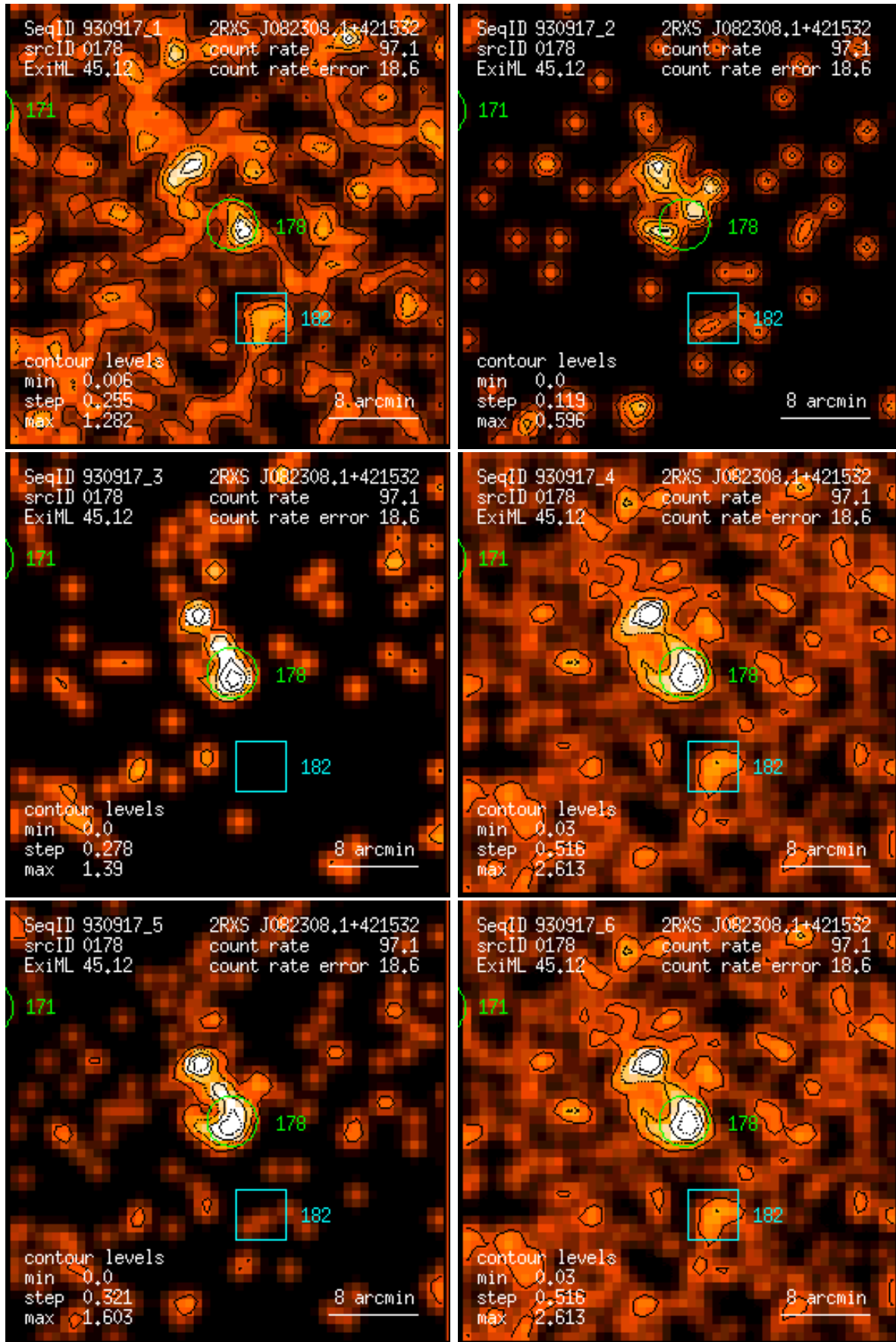
Figure 178: RASS 930917: detection 0178: band rate images, Gaussian filter: (1) PSPC channels 11 – 41, (2) 52 – 90, (3) 91 – 201, (4) 11 – 235, (5) 52 – 201, (6) 11 – 201. Broad band rates in counts/ks. Band rate contour levels in counts/ks/arcmin 2 .
