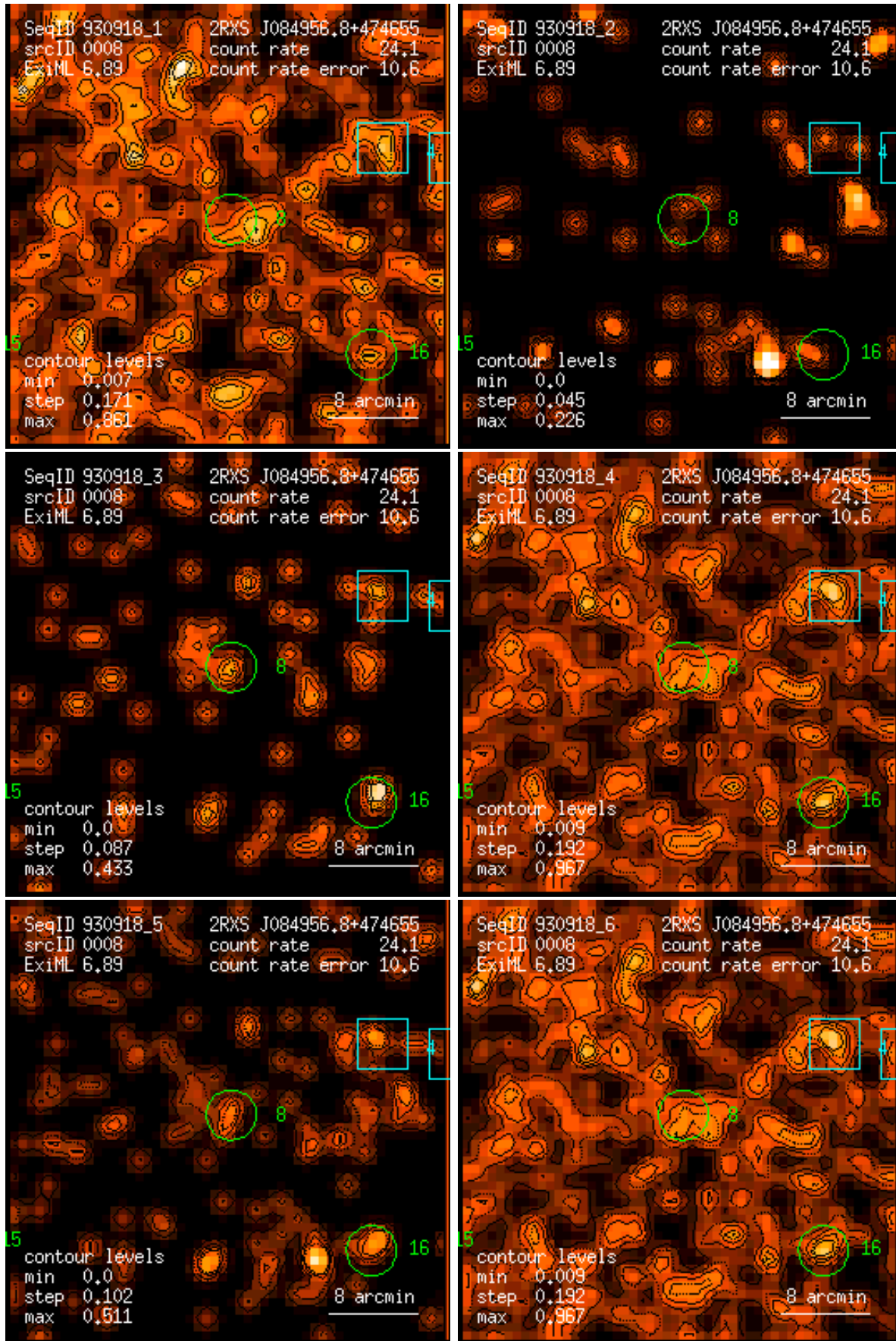
Figure 8: RASS 930918: detection 0008: band rate images, Gaussian filter: (1) PSPC channels 11 – 41, (2) 52 – 90, (3) 91 – 201, (4) 11 – 235, (5) 52 – 201, (6) 11 – 201. Broad band rates in counts/ks. Band rate contour levels in counts/ks/arcmin 2 .
