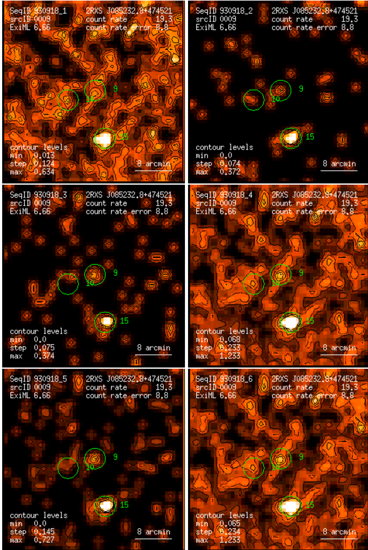
Figure 9: RASS 930918: detection 0009: band rate images, Gaussian filter: (1) PSPC channels 11 – 41, (2) 52 – 90, (3) 91 – 201, (4) 11 – 235, (5) 52 – 201, (6) 11 – 201. Broad band rates in counts/ks. Band rate contour levels in counts/ks/arcmin 2 .
