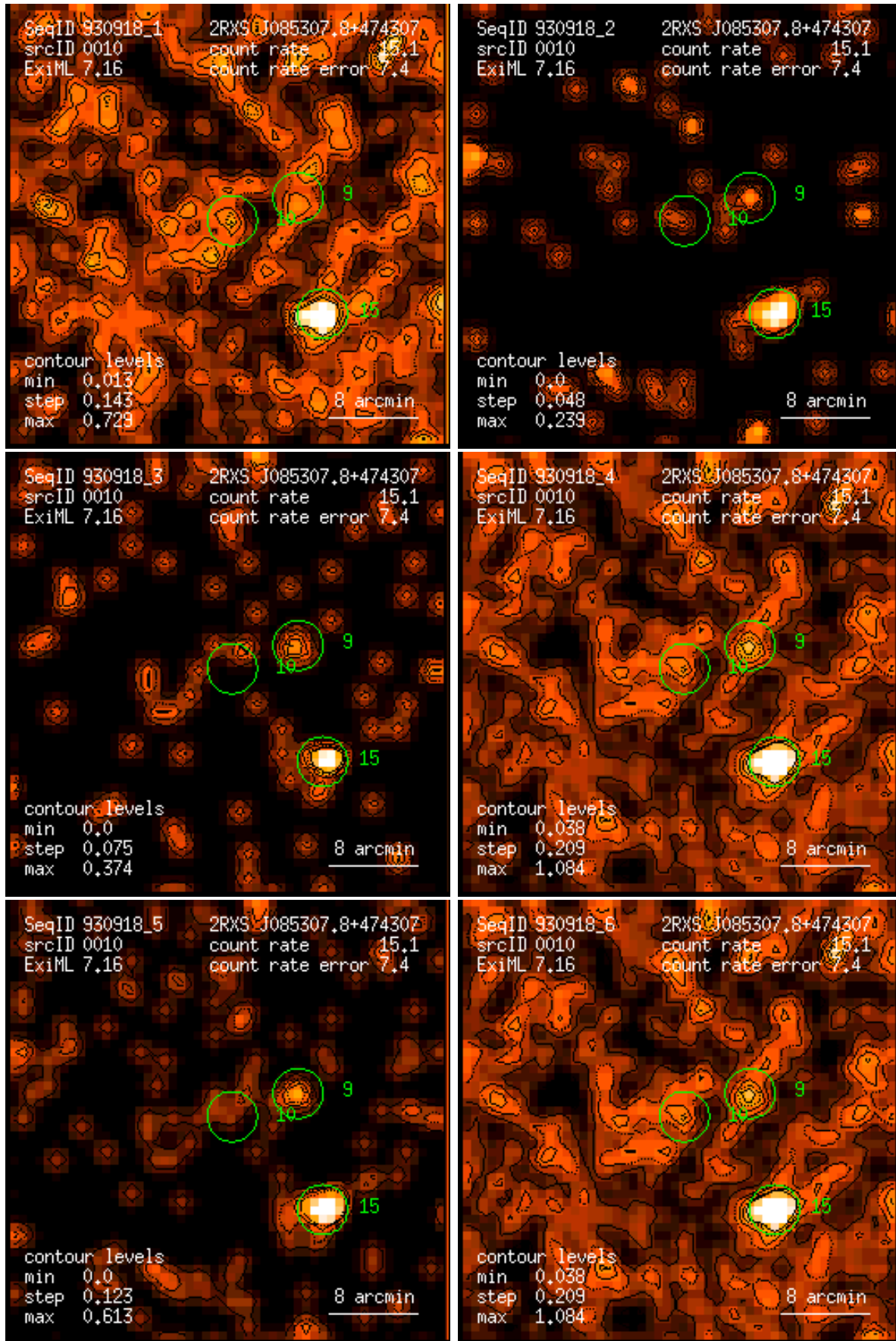
Figure 10: RASS 930918: detection 0010: band rate images, Gaussian filter: (1) PSPC channels 11 – 41, (2) 52 – 90, (3) 91 – 201, (4) 11 – 235, (5) 52 – 201, (6) 11 – 201. Broad band rates in counts/ks. Band rate contour levels in counts/ks/arcmin 2 .
