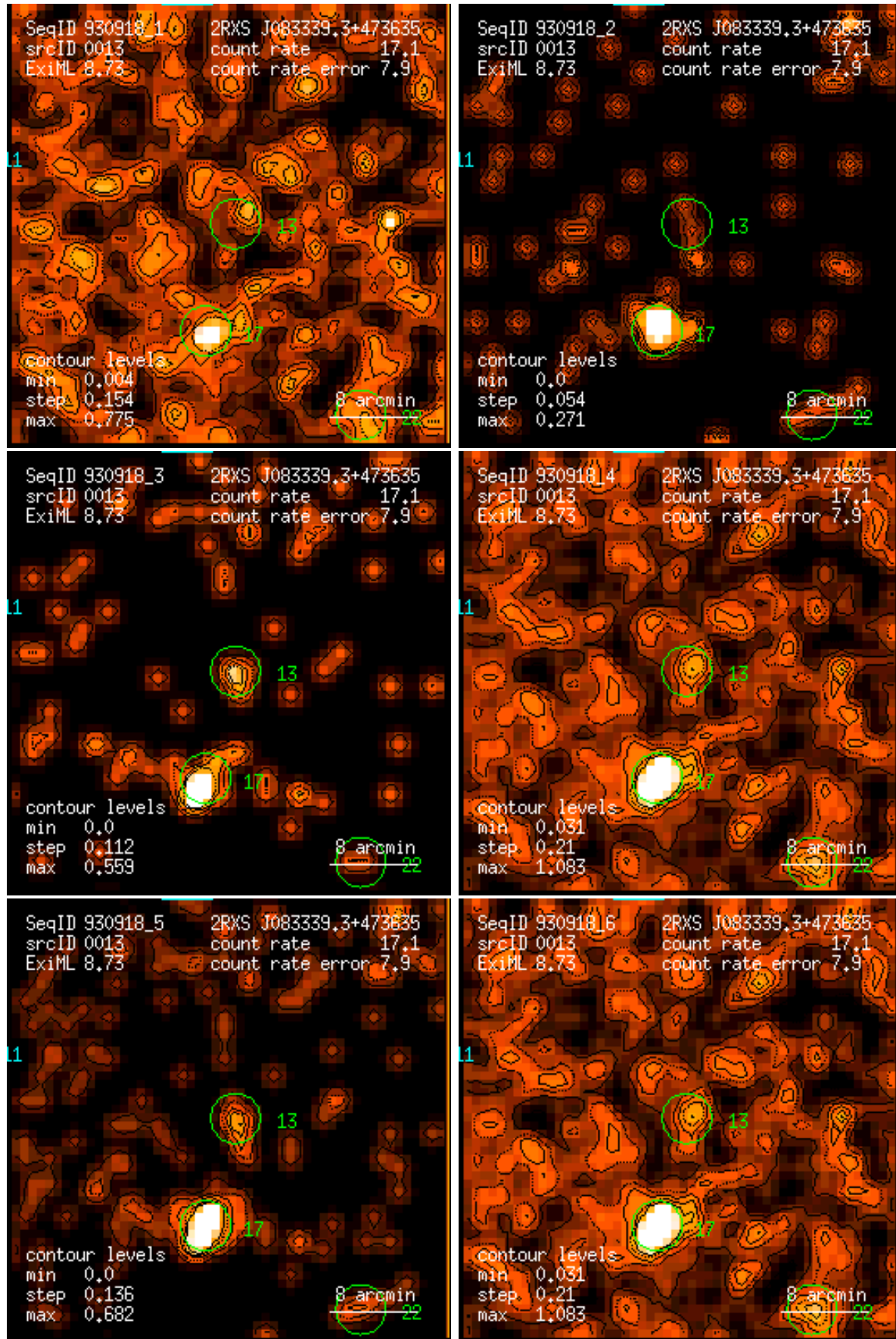
Figure 13: RASS 930918: detection 0013: band rate images, Gaussian filter: (1) PSPC channels 11 – 41, (2) 52 – 90, (3) 91 – 201, (4) 11 – 235, (5) 52 – 201, (6) 11 – 201. Broad band rates in counts/ks. Band rate contour levels in counts/ks/arcmin 2 .
