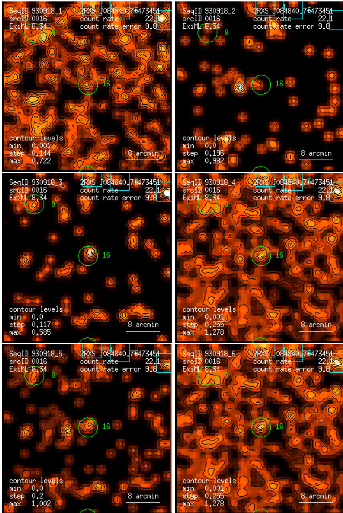
Figure 16: RASS 930918: detection 0016: band rate images, Gaussian filter: (1) PSPC channels 11 – 41, (2) 52 – 90, (3) 91 – 201, (4) 11 – 235, (5) 52 – 201, (6) 11 – 201. Broad band rates in counts/ks. Band rate contour levels in counts/ks/arcmin 2 .
