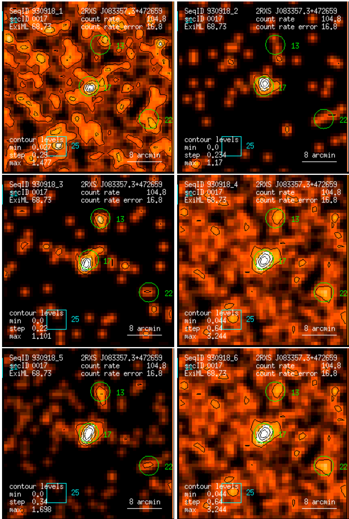
Figure 17: RASS 930918: detection 0017: band rate images, Gaussian filter: (1) PSPC channels 11 – 41, (2) 52 – 90, (3) 91 – 201, (4) 11 – 235, (5) 52 – 201, (6) 11 – 201. Broad band rates in counts/ks. Band rate contour levels in counts/ks/arcmin 2 .
