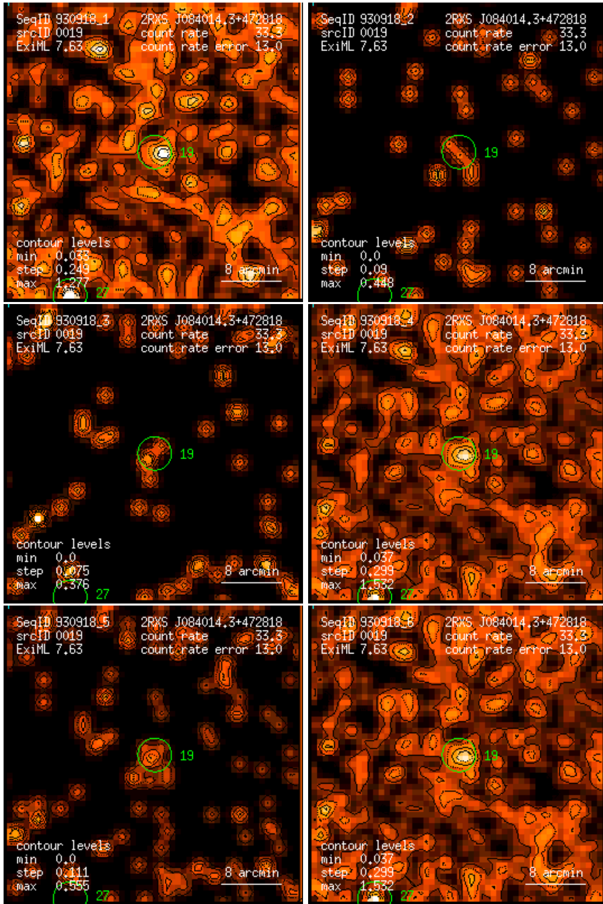
Figure 19: RASS 930918: detection 0019: band rate images, Gaussian filter: (1) PSPC channels 11 – 41, (2) 52 – 90, (3) 91 – 201, (4) 11 – 235, (5) 52 – 201, (6) 11 – 201. Broad band rates in counts/ks. Band rate contour levels in counts/ks/arcmin 2 .
