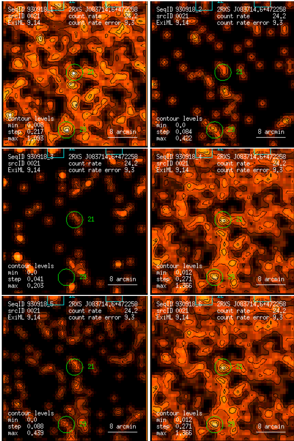
Figure 21: RASS 930918: detection 0021: band rate images, Gaussian filter: (1) PSPC channels 11 – 41, (2) 52 – 90, (3) 91 – 201, (4) 11 – 235, (5) 52 – 201, (6) 11 – 201. Broad band rates in counts/ks. Band rate contour levels in counts/ks/arcmin 2 .
