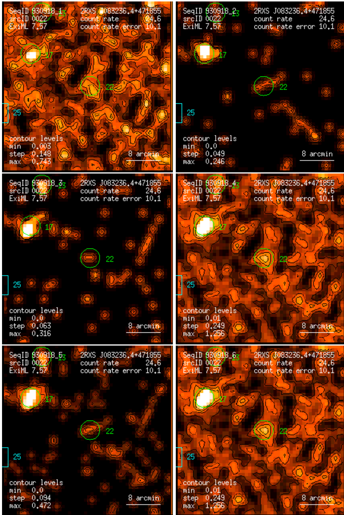
Figure 22: RASS 930918: detection 0022: band rate images, Gaussian filter: (1) PSPC channels 11 – 41, (2) 52 – 90, (3) 91 – 201, (4) 11 – 235, (5) 52 – 201, (6) 11 – 201. Broad band rates in counts/ks. Band rate contour levels in counts/ks/arcmin 2 .
