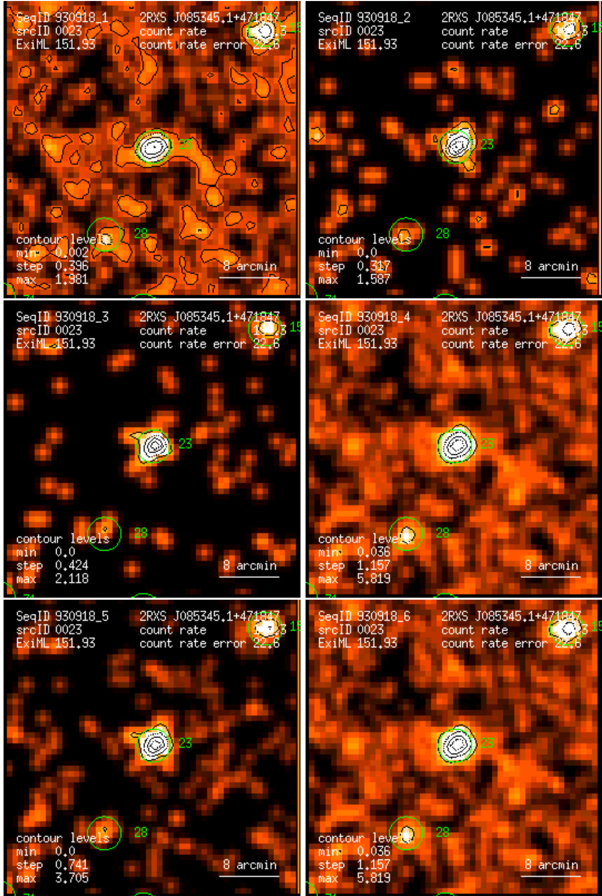
Figure 23: RASS 930918: detection 0023: band rate images, Gaussian filter: (1) PSPC channels 11 – 41, (2) 52 – 90, (3) 91 – 201, (4) 11 – 235, (5) 52 – 201, (6) 11 – 201. Broad band rates in counts/ks. Band rate contour levels in counts/ks/arcmin 2 .
