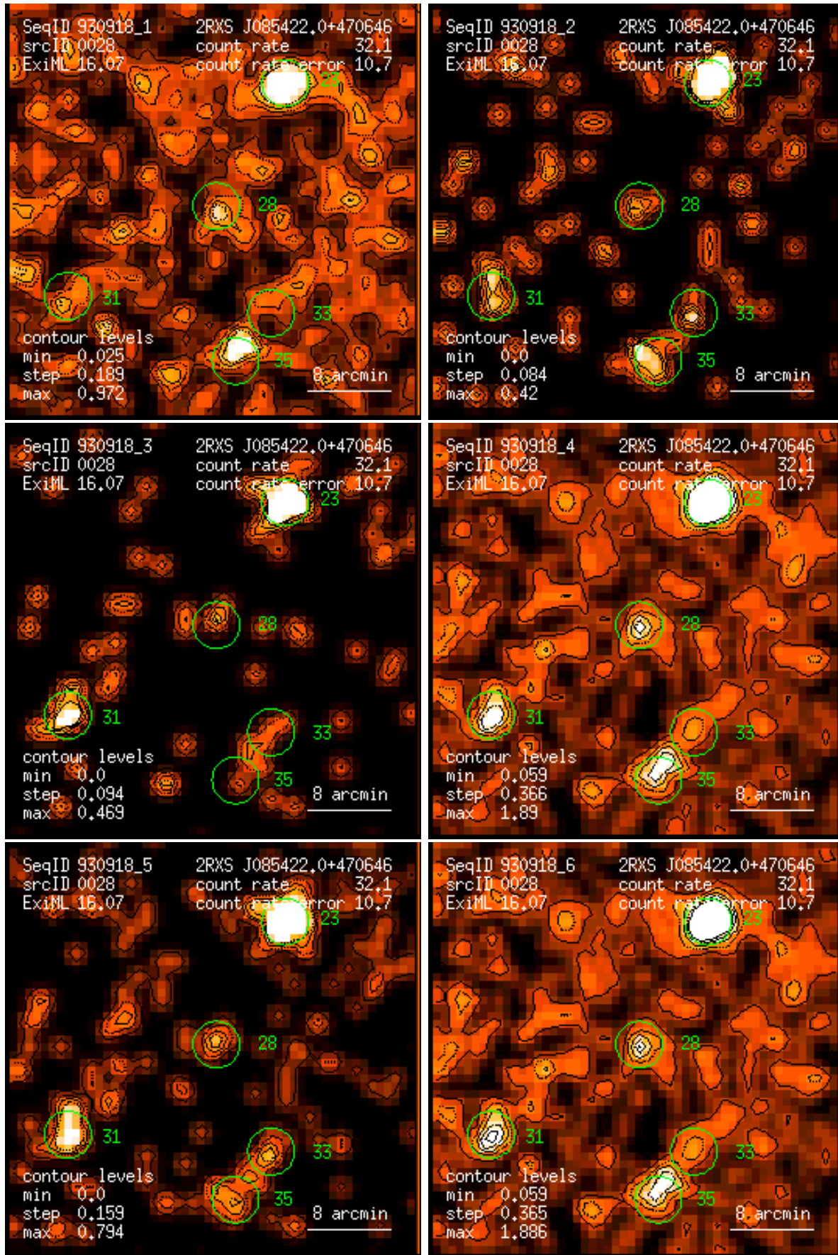
Figure 28: RASS 930918: detection 0028: band rate images, Gaussian filter: (1) PSPC channels 11 – 41, (2) 52 – 90, (3) 91 – 201, (4) 11 – 235, (5) 52 – 201, (6) 11 – 201. Broad band rates in counts/ks. Band rate contour levels in counts/ks/arcmin 2 .
