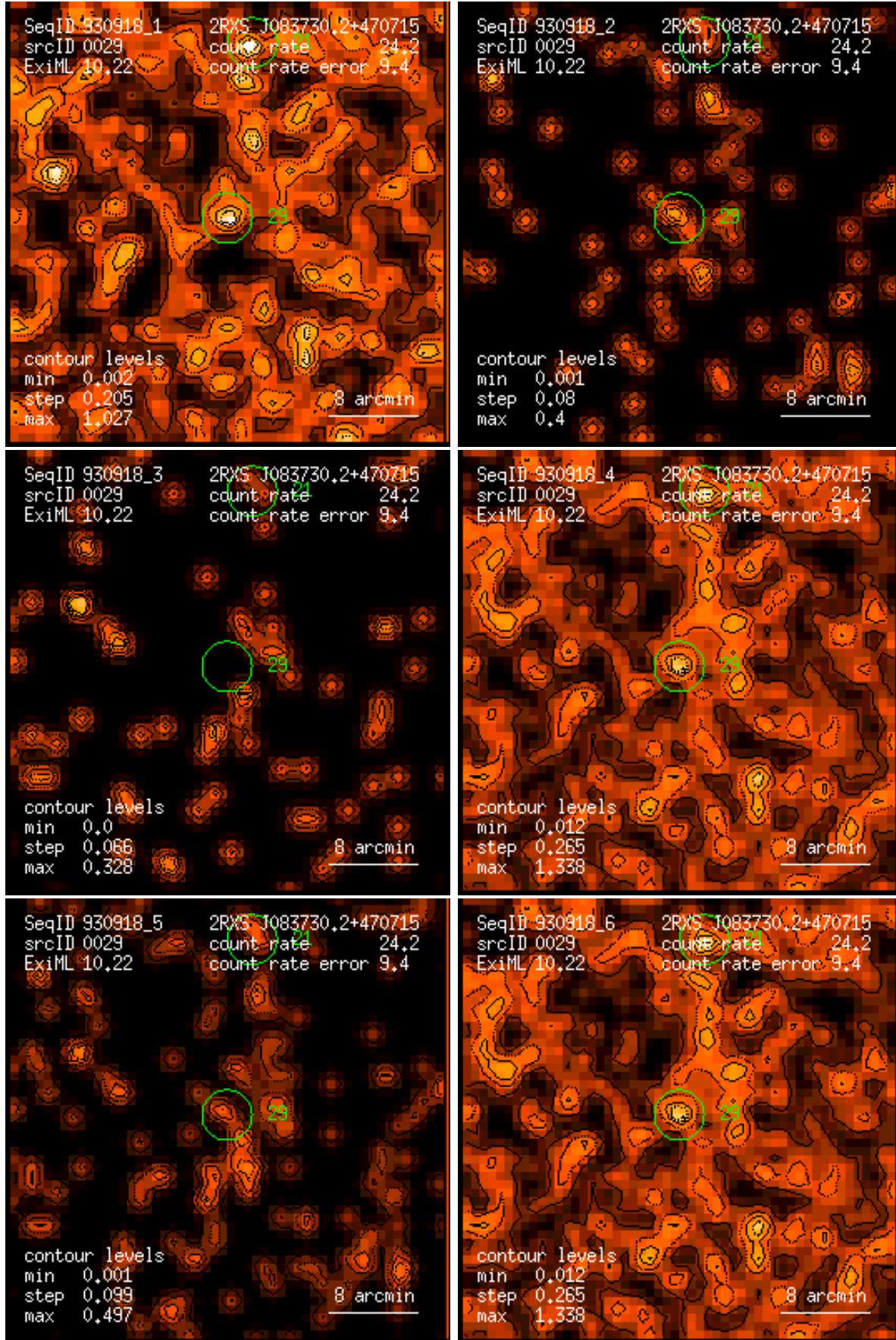
Figure 29: RASS 930918: detection 0029: band rate images, Gaussian filter: (1) PSPC channels 11 – 41, (2) 52 – 90, (3) 91 – 201, (4) 11 – 235, (5) 52 – 201, (6) 11 – 201. Broad band rates in counts/ks. Band rate contour levels in counts/ks/arcmin 2 .
