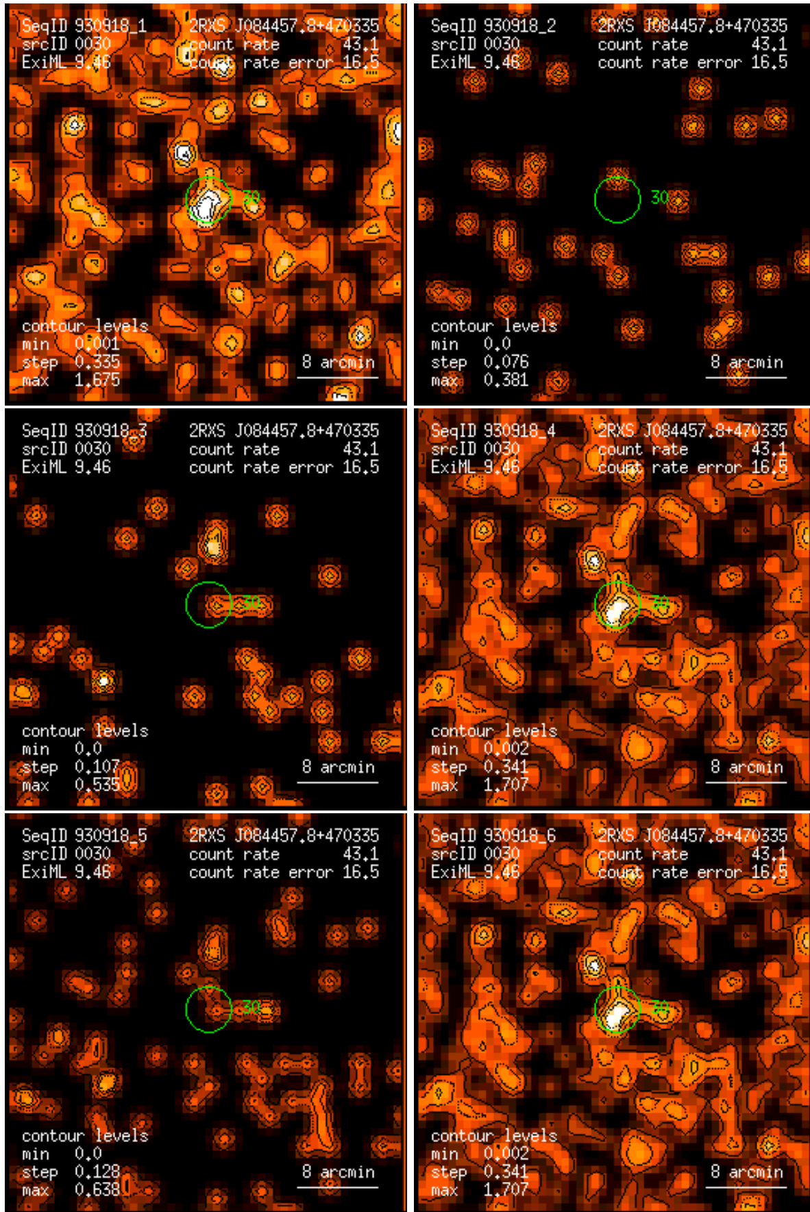
Figure 30: RASS 930918: detection 0030: band rate images, Gaussian filter: (1) PSPC channels 11 – 41, (2) 52 – 90, (3) 91 – 201, (4) 11 – 235, (5) 52 – 201, (6) 11 – 201. Broad band rates in counts/ks. Band rate contour levels in counts/ks/arcmin 2 .
