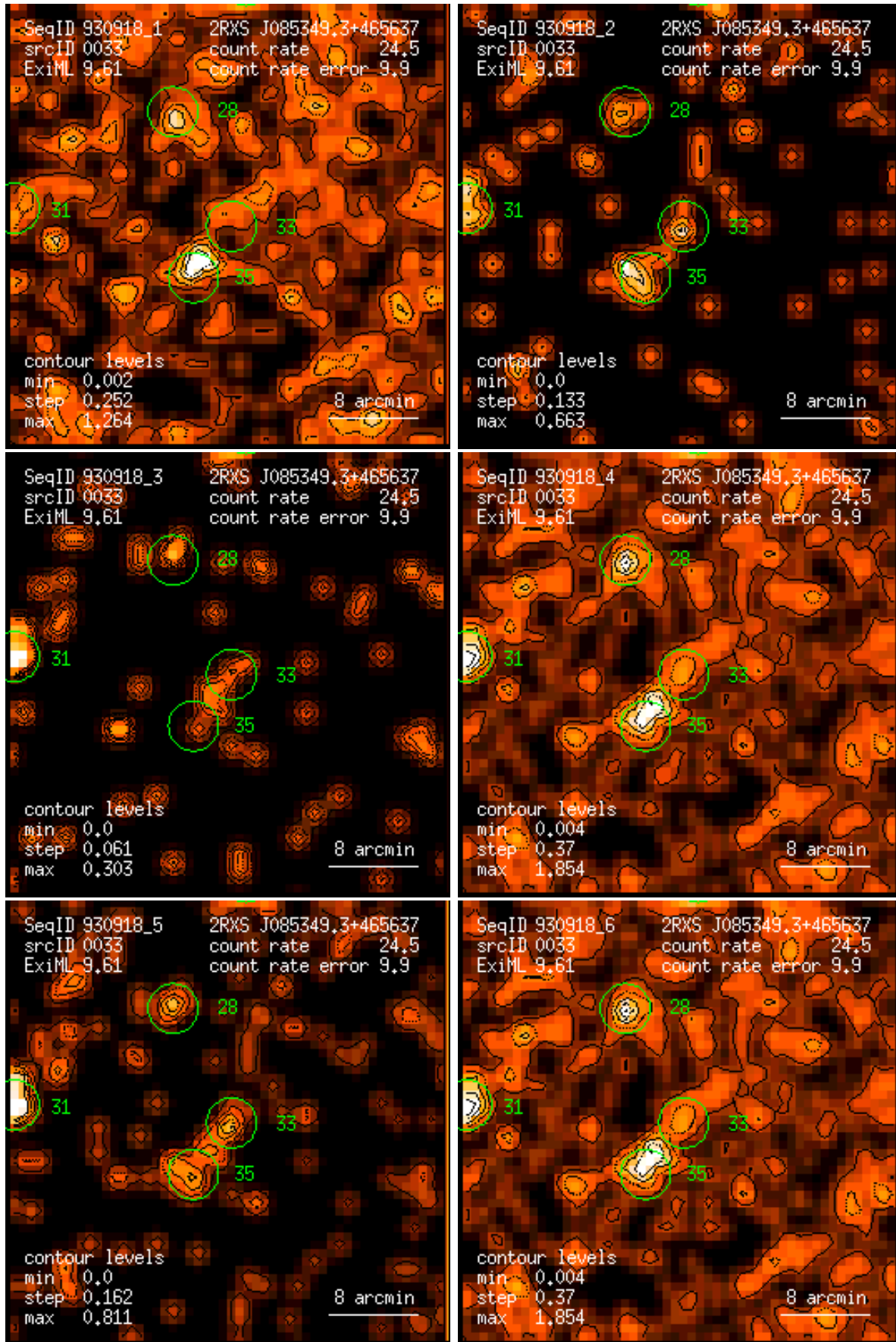
Figure 33: RASS 930918: detection 0033: band rate images, Gaussian filter: (1) PSPC channels 11 – 41, (2) 52 – 90, (3) 91 – 201, (4) 11 – 235, (5) 52 – 201, (6) 11 – 201. Broad band rates in counts/ks. Band rate contour levels in counts/ks/arcmin 2 .
