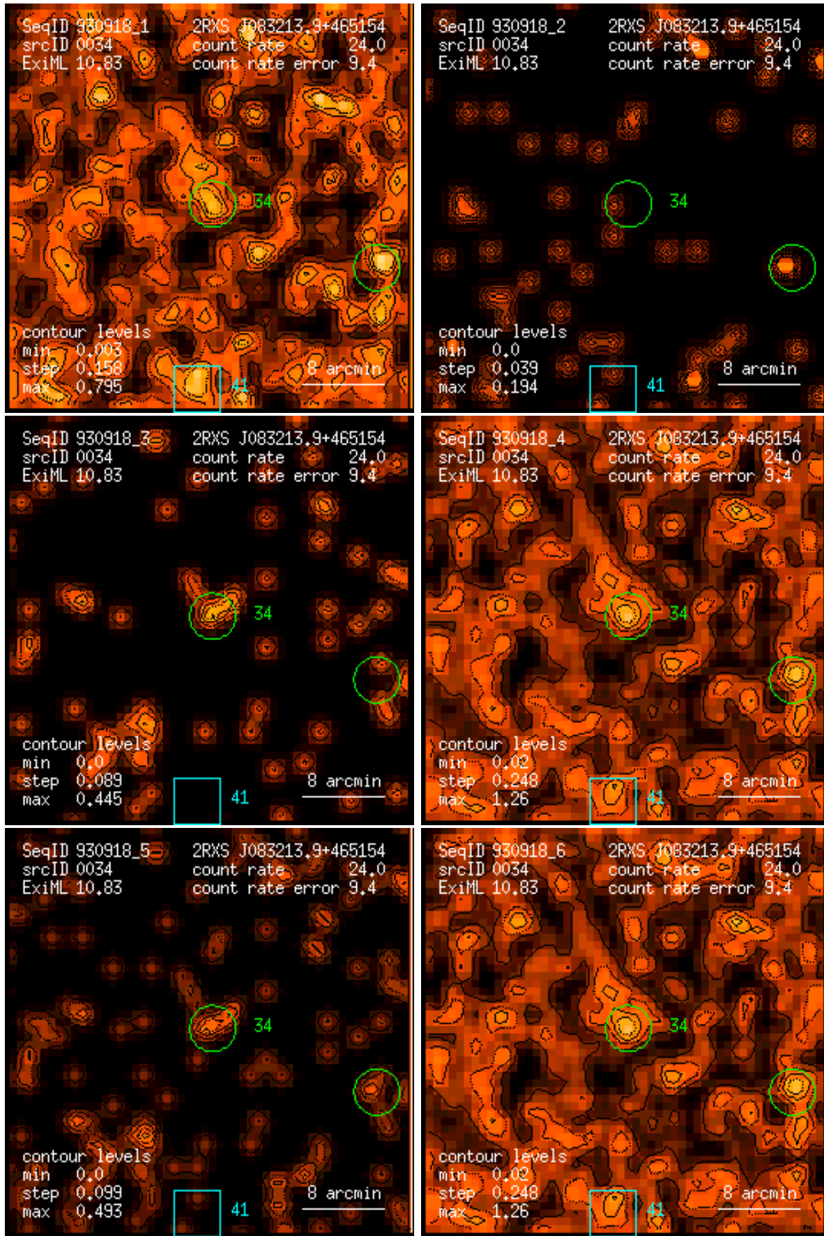
Figure 34: RASS 930918: detection 0034: band rate images, Gaussian filter: (1) PSPC channels 11 – 41, (2) 52 – 90, (3) 91 – 201, (4) 11 – 235, (5) 52 – 201, (6) 11 – 201. Broad band rates in counts/ks. Band rate contour levels in counts/ks/arcmin 2 .
